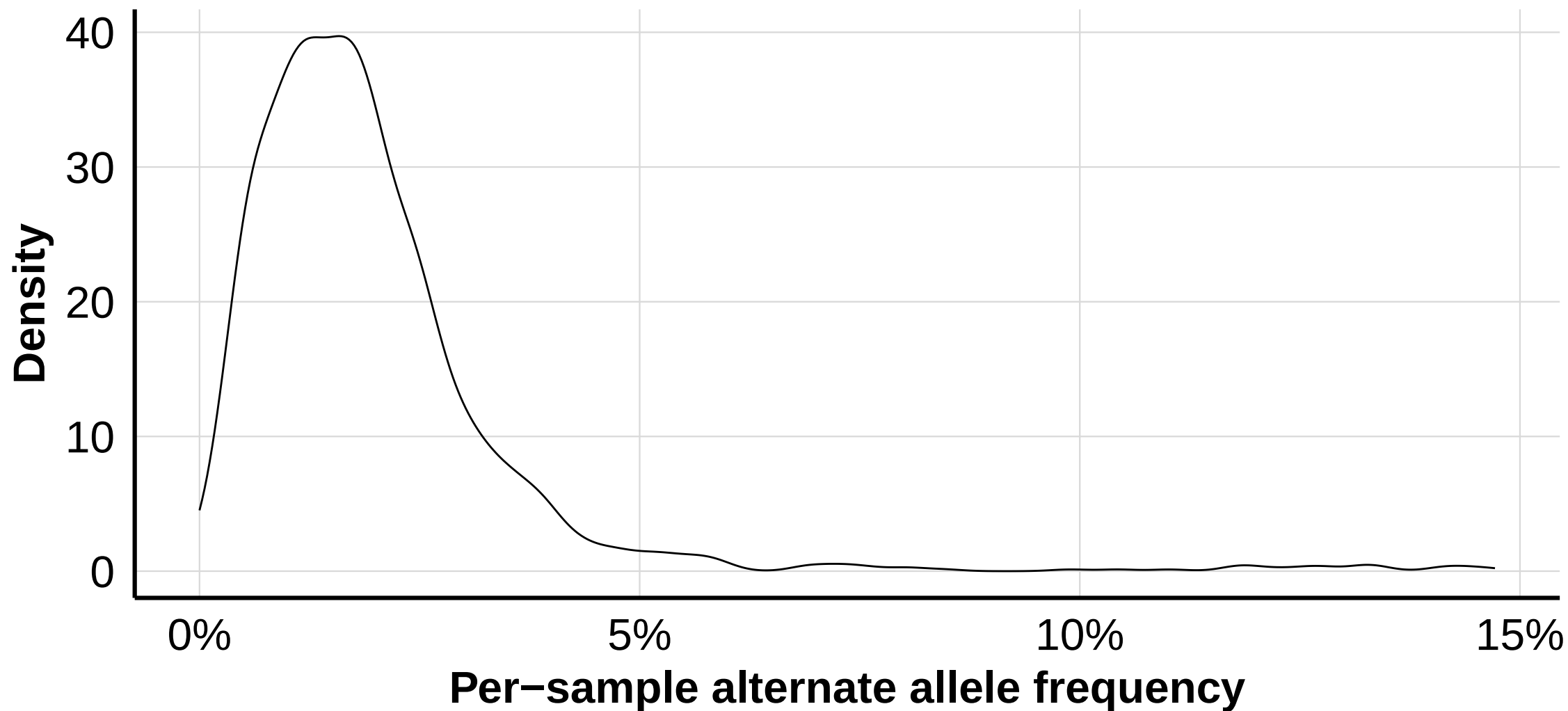
Per-sample alt allele frequency: unimputed
