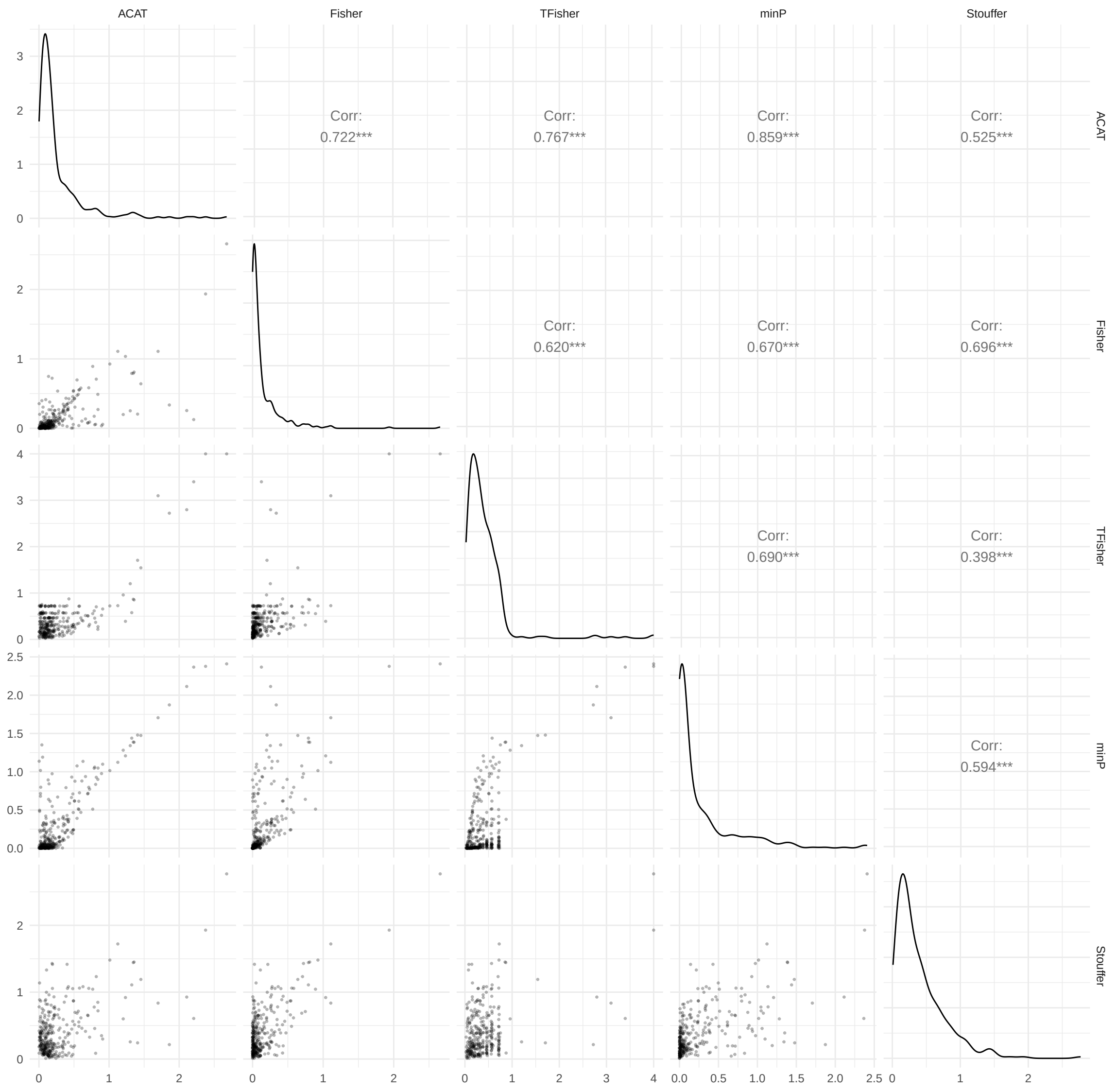
Pairwise Comparison of -\log_{10}(p) Across Methods
