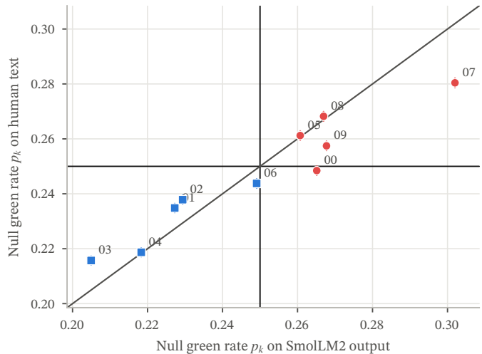
(b) Key ranking agrees, \rho = +0.94
