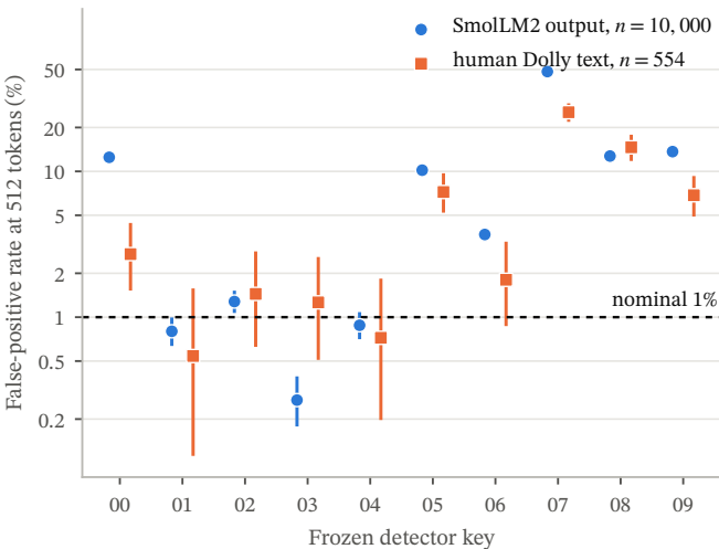
(a) The same keys on human-written text
