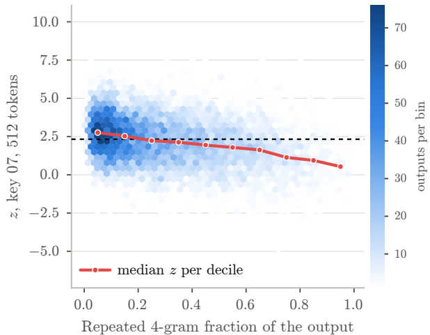
(b) Worst key, Spearman \rho = -0.29
