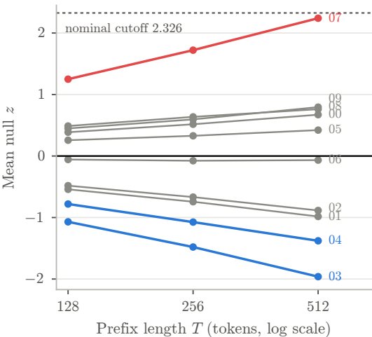
(a) Offsets grow as \sqrt{T}
