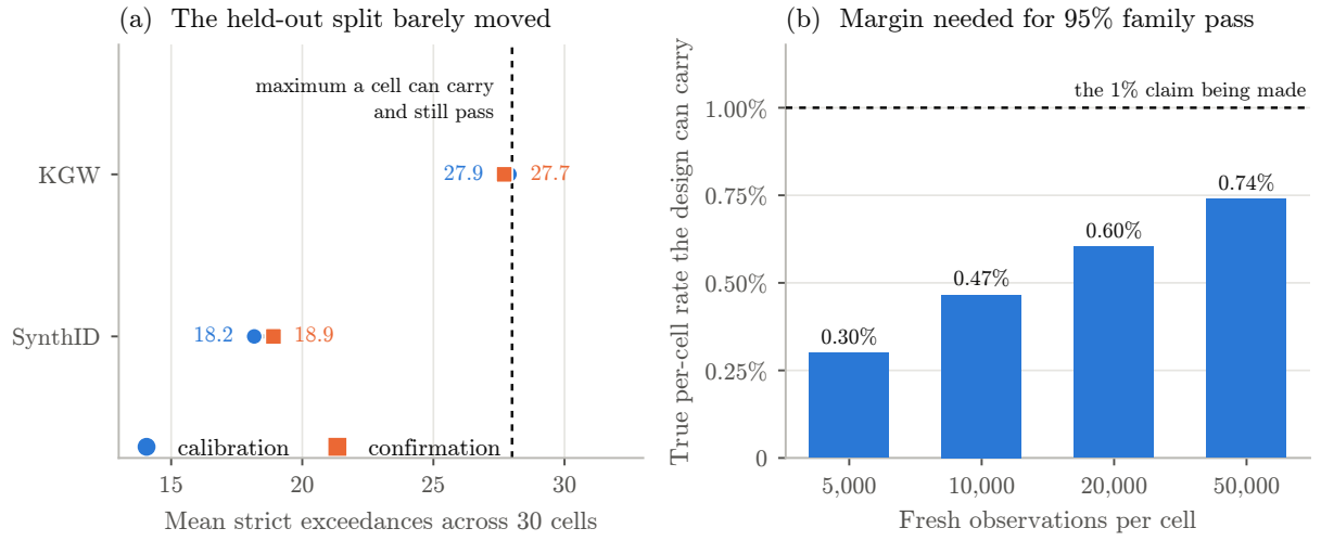
Figure 7: (a) Mean strict exceedances across the 30 key-by-length cells of each scheme, on the calibration split and on the disjoint confirmation split, against the largest count a cell could carry and still pass. KGW’s pair sits on the boundary and barely moves, so the gate failure is not a held-out shift. (b) Prospective union-bound planning: the largest true per-cell rate compatible with at least 95% probability that all 60 cells pass, by fresh sample size. These are design scenarios, not replacement thresholds.
