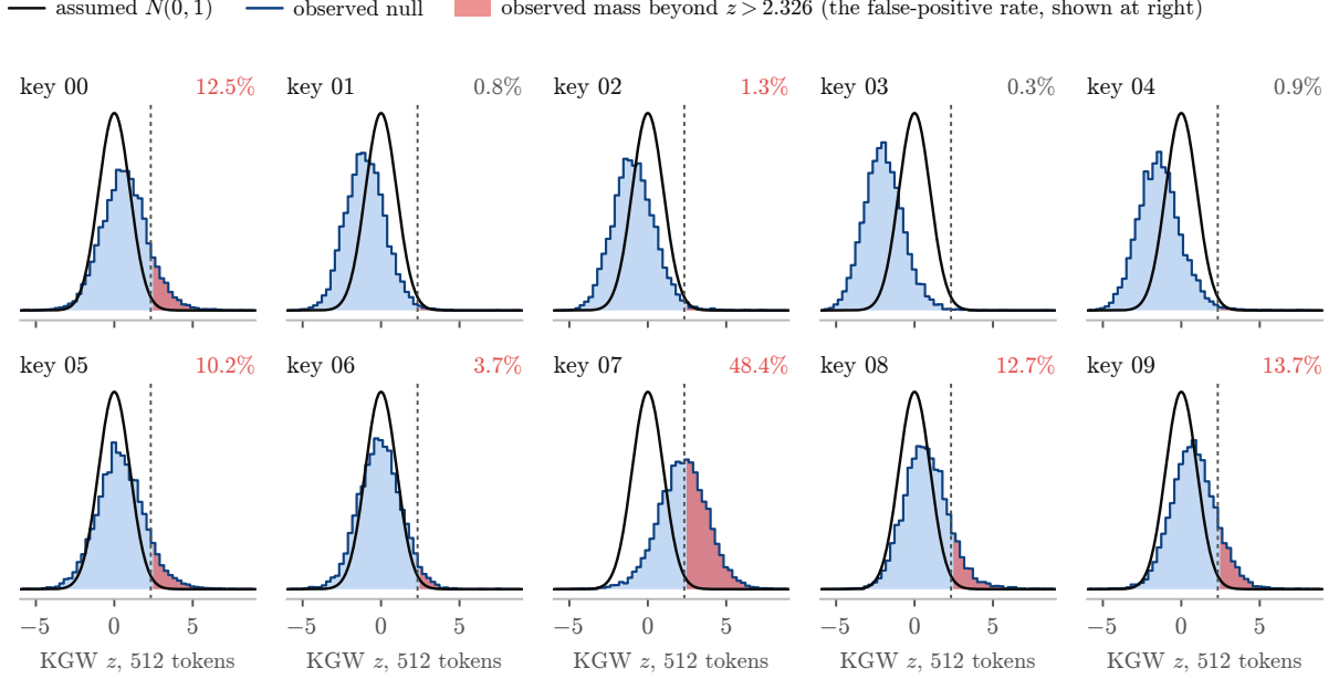
Figure 3: Null distribution of the KGW z statistic at 512 tokens for each of the ten keys, n = 10,000 , against the assumed standard normal (solid) and the nominal cutoff (dashed). The shaded area past the cutoff is the mass this key puts beyond the nominal 1% threshold; the percentage at each panel’s top right is that cell’s false-positive rate. Under the assumed null every panel would show the same 1%.
