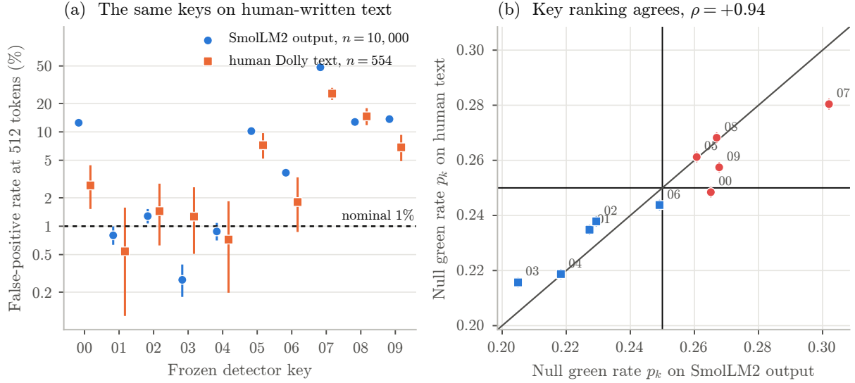
Figure 6: (a) False-positive rate at the nominal threshold and 512 tokens for the same ten keys on SmolLM2 output ( n = 10,000 ) and on human-written Dolly passages ( n = 554 ), exact 95% intervals, log scale. The human intervals are wide because the 512-token human cell is small. (b) Per-key null green rate on human text against the same quantity on model output, with exact intervals on both axes; the diagonal is equality and the rules mark \gamma = 0.25 . Colour is the same side-of- \gamma encoding as Figure 4a.
