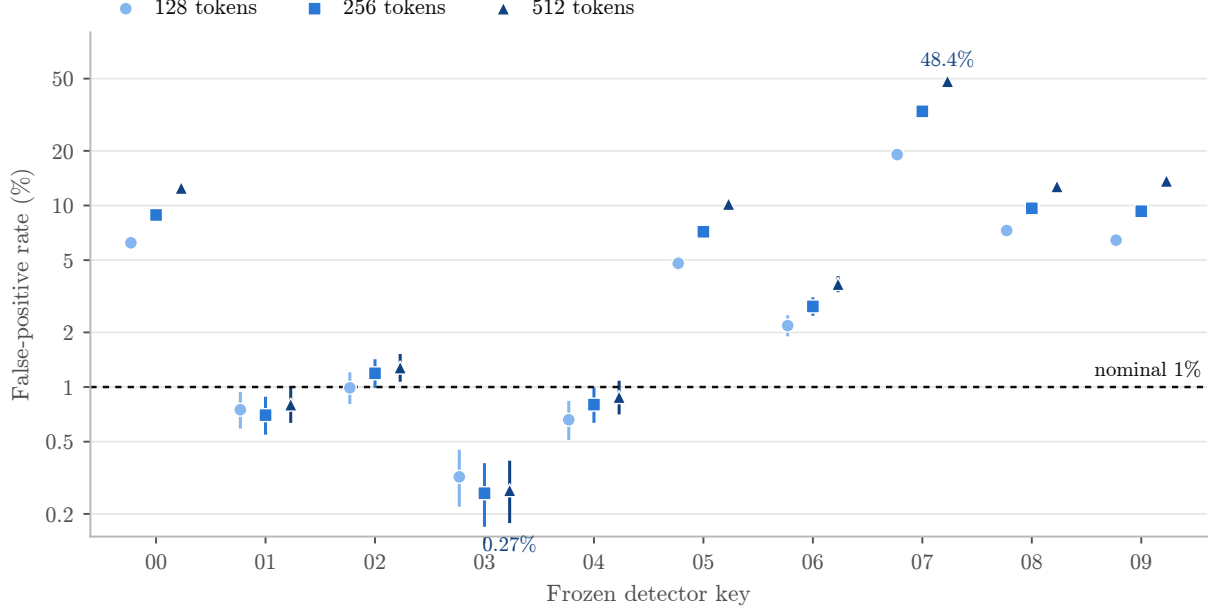
Figure 1: Canonical KGW SelfHash false-positive rate by frozen detector key and prefix length at the nominal z > 2.326 threshold, n = 10,000 unwatermarked SmolLM2 outputs per cell, exact 95% intervals, log scale. Prefix length is shaded light to dark. Keys are categorical and are paired within texts, so the points are not independent across keys.
