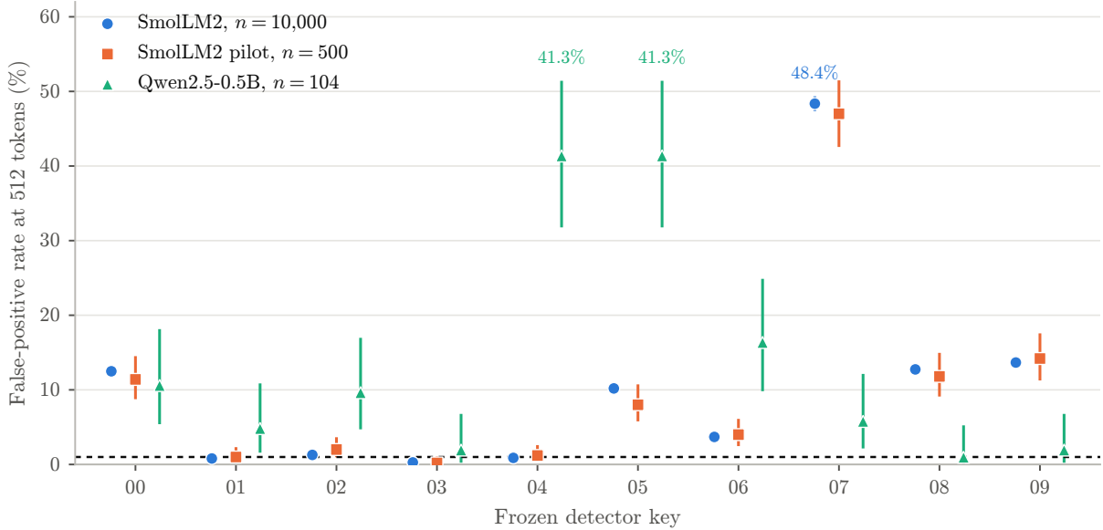
Figure 2: The same ten keys at 512 tokens in three null runs: the primary SmolLM2 corpus ( n = 10,000 ), the SmolLM2 pilot ( n = 500 ), and the Qwen2.5-0.5B replication ( n = 104 ). The two SmolLM2 runs agree; the Qwen run inflates different keys.
