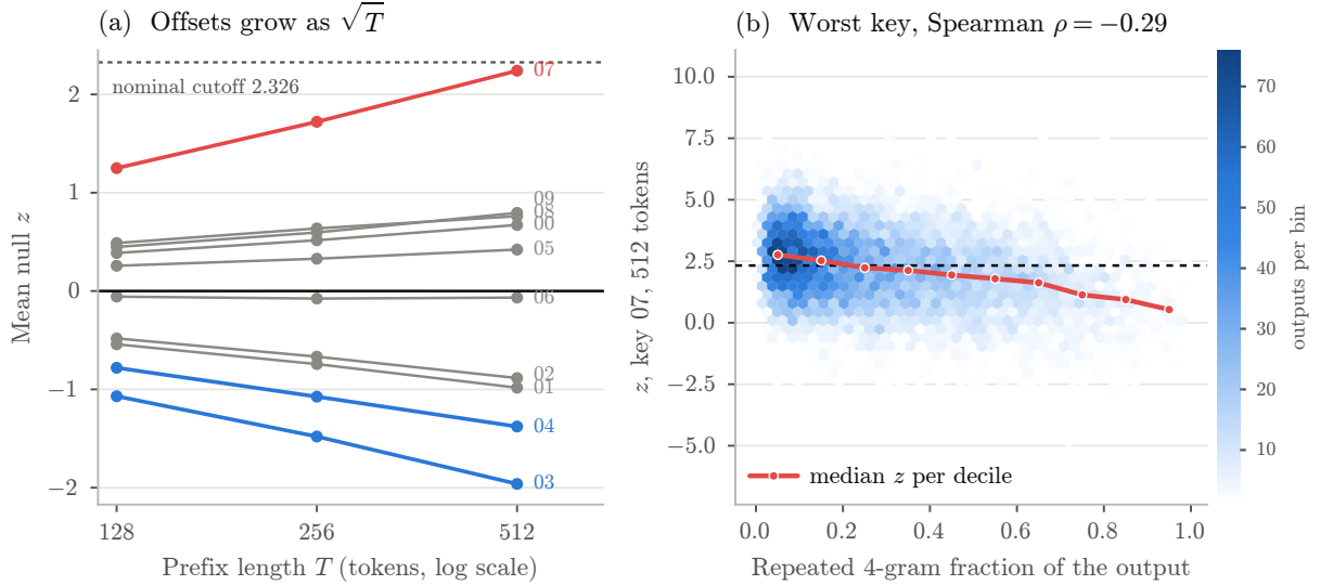
Figure 5: (a) Mean null z per key against prefix length on a log scale; the offsets grow as \sqrt{T} , away from zero in both directions, and only the keys ending beyond |z| = 1 are coloured. (b) Density of per-output z for key 07 at 512 tokens against the output’s repeated-4-gram fraction, n = 10,000 , with the median per decile; more repetition goes with lower z , not higher.
