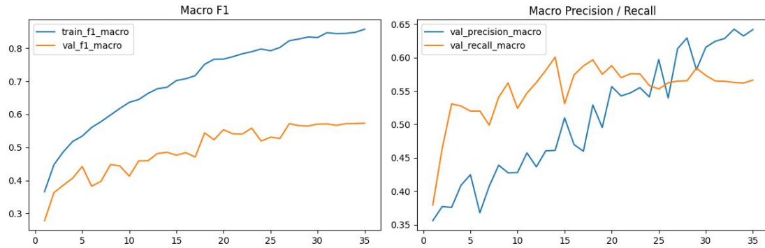
Figure 4: Training and validation metric curves for cnn_residual_fullprotocol
