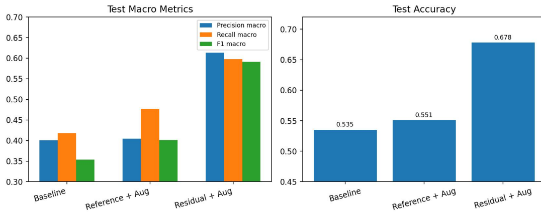
Figure 5: Test-set metric comparison across CNN variants ( Accuracy , Precision_{macro} , Recall_{macro} , F1_{macro} ).
