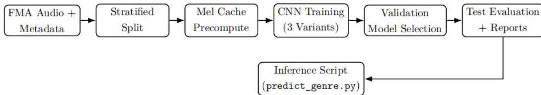
Figure 3: End-to-end ML pipeline used in this project
