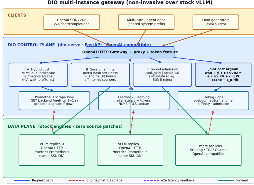
Fig. 1 DIO multi-instance gateway. OpenAI clients hit dio-serve; the control plane combines NLMS ranking, Prometheus /metrics scrape, session affinity, and decoupled admission over stock vLLM replicas (no engine patches, no multi-SKU assumption).
