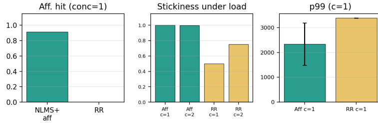
Fig. 5 Real dual-T4 multi-turn affinity vs. RR ( n=5 ). Hit rate, stickiness, and p99 e2e.
