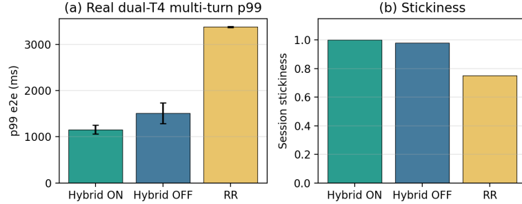
Fig. 4 Real dual-T4 multi-turn hybrid suite ( n=5 ). (a) p99 e2e; (b) session stickiness. Hybrid ON beats hybrid OFF and RR.
