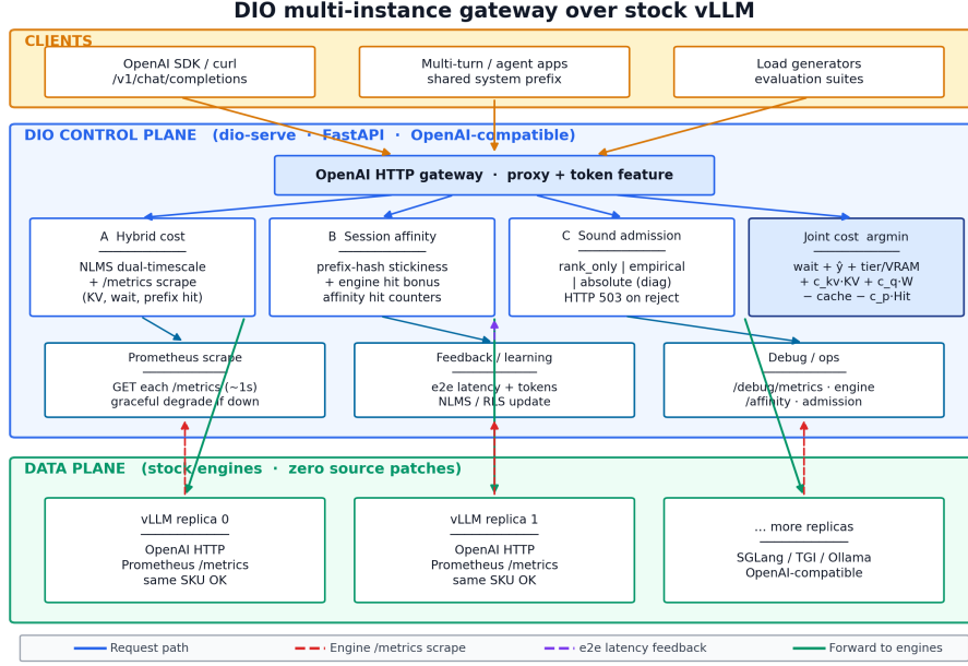
Fig. 1 DIO multi-instance gateway. OpenAI clients call dio-serve ; the control plane combines NLMS ranking, Prometheus /metrics scrape, session affinity, and decoupled admission over stock vLLM replicas (no engine patches; no multi-SKU assumption).
