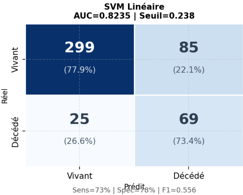
Figure 5.9 – Confusion matrix — SVM Linéaire (AUC = 0.8235, seuil = 0.238).
