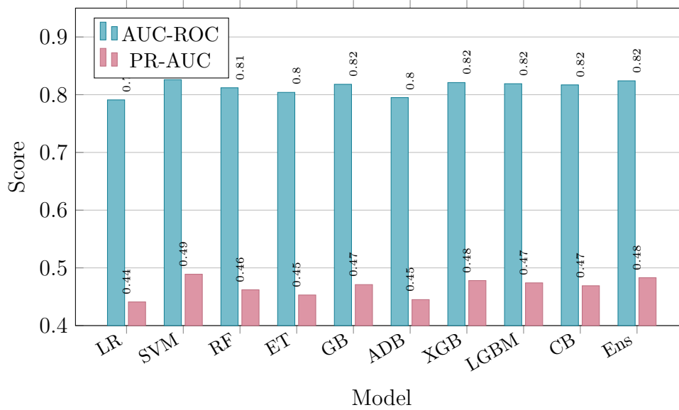
Figure 5.1 – AUC-ROC and PR-AUC comparison across all evaluated models (HD-478 cohort, 10-fold stratified CV). SVM achieves the highest scores on both metrics.
