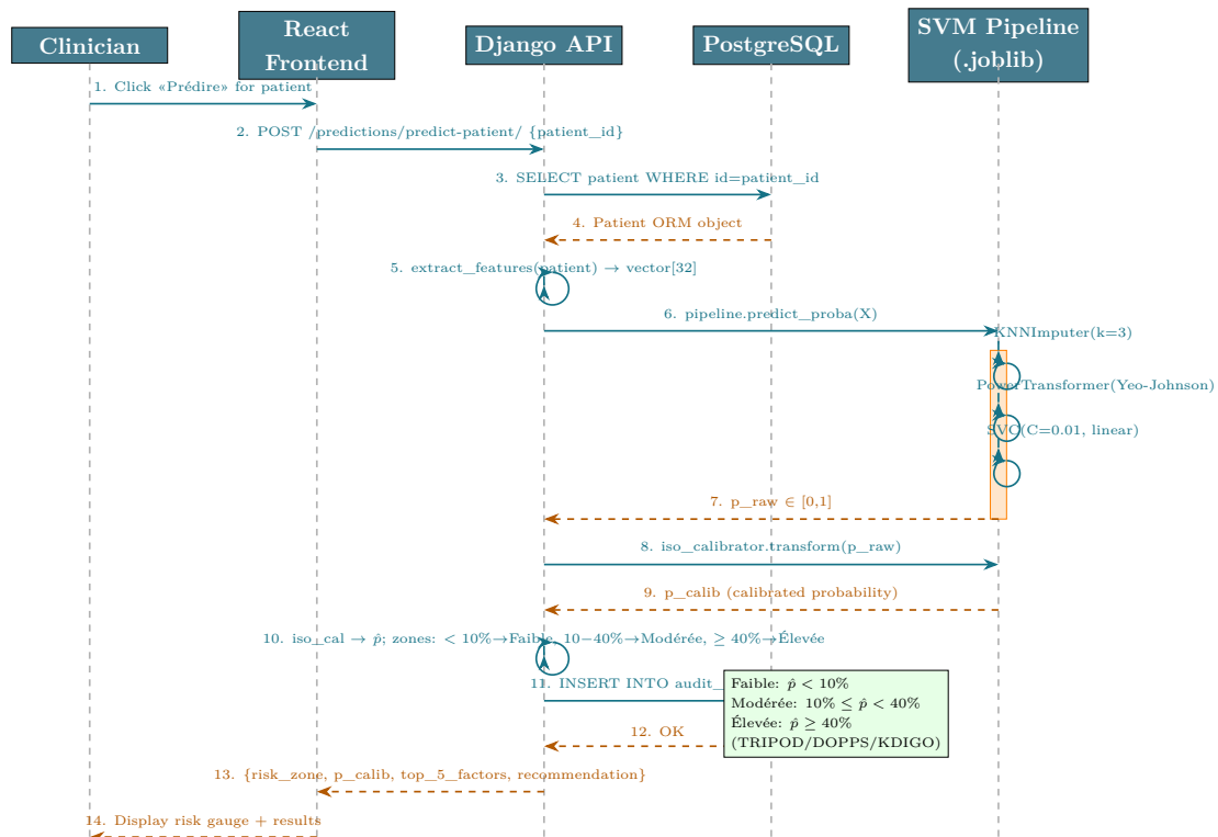
Figure 6.21 – Sequence Diagram 3 — Mortality Risk Prediction workflow
