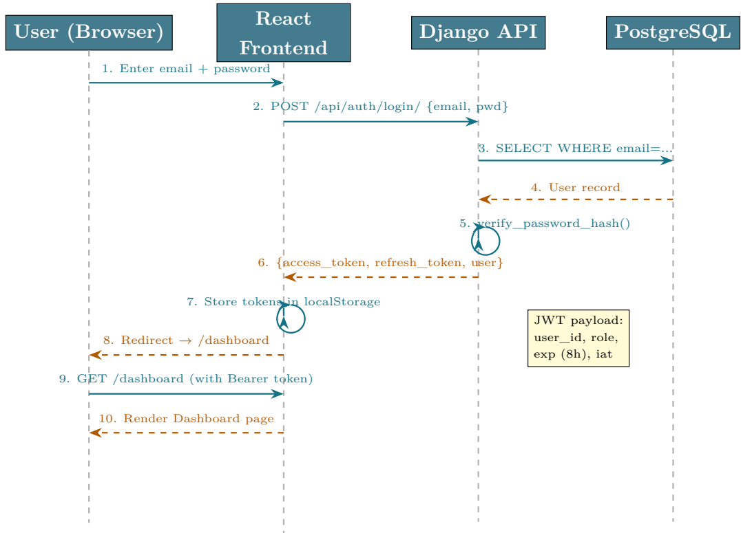
Figure 6.19 – Sequence Diagram 1 — JWT Authentication flow
