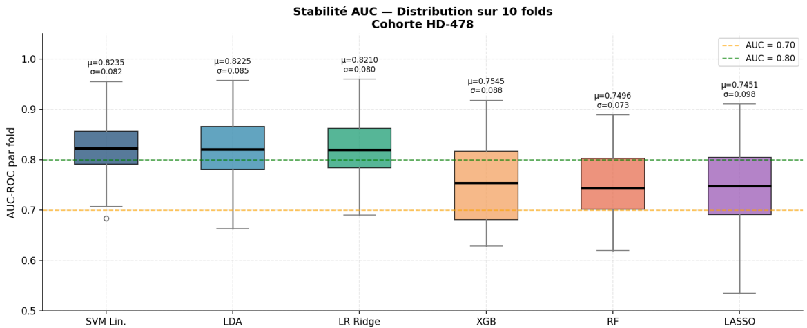
Figure 5.8 – Boxplot of AUC-ROC scores across 10 stratified cross-validation folds for each model, illustrating variance and stability of model performance.
