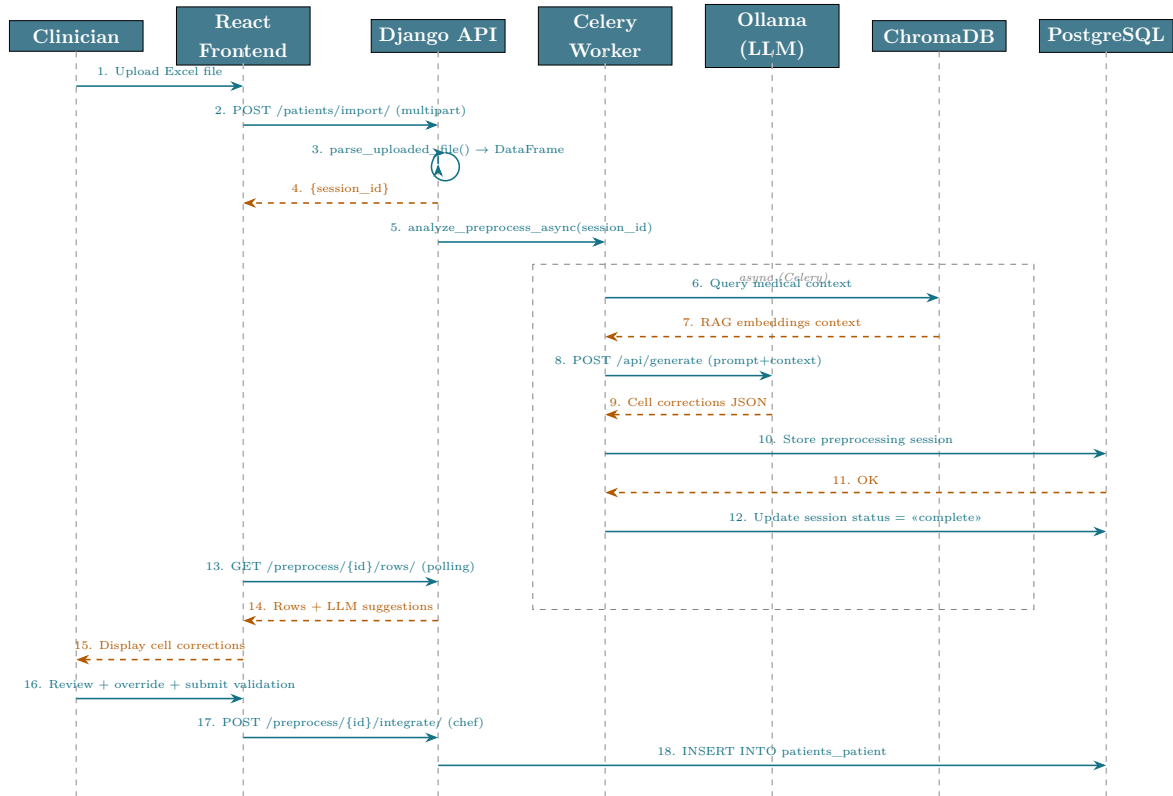
Figure 6.20 – Sequence Diagram 2 — Patient Import and LLM Preprocessing
