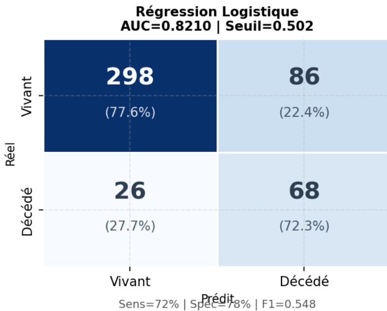
Figure 5.10 – Confusion matrix — R  gression Logistique (AUC = 0.8210, seuil = 0.502).
