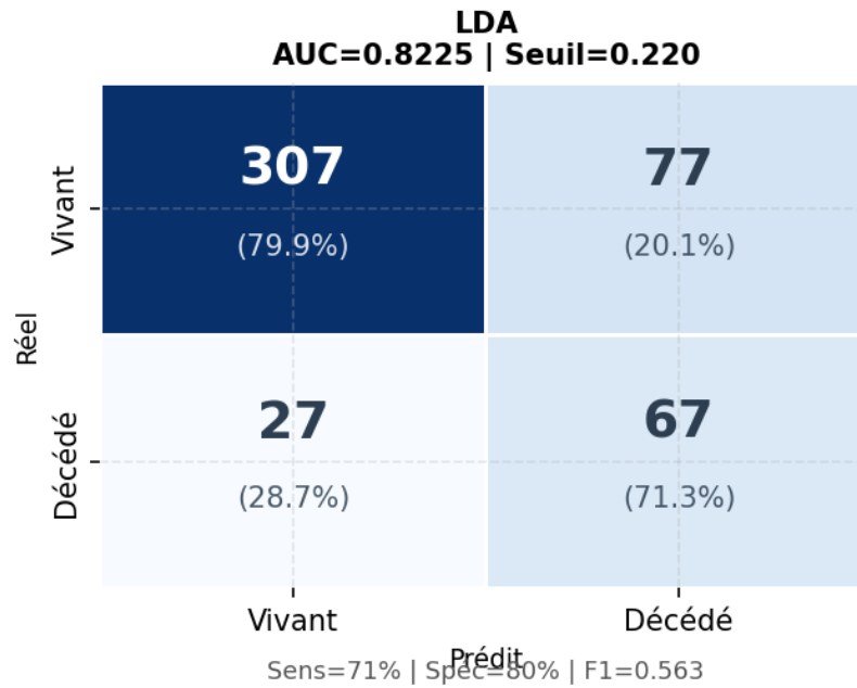
Figure 5.9 – Confusion matrix — LDA (AUC = 0.8225, seuil = 0.220).
