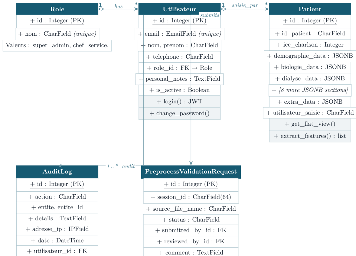
Figure 6.2 – UML Class Diagram — main Django models
