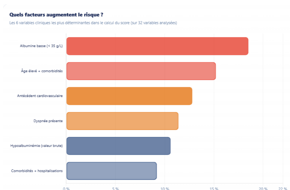
Figure 6.45 — Top contributing risk factors — mean SVM feature weights across the cohort, ranked by absolute importance
