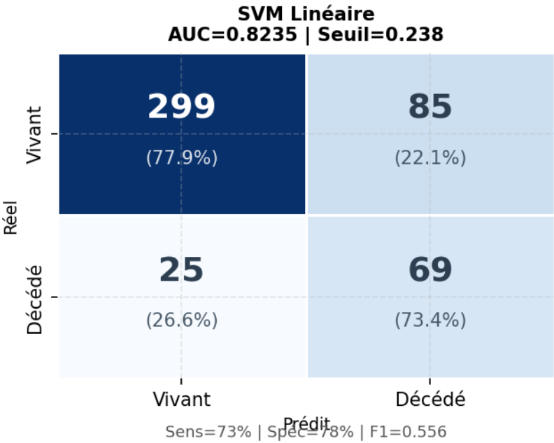
Figure 5.8 – Confusion matrix — SVM Linéaire (AUC = 0.8235, seuil = 0.238).
