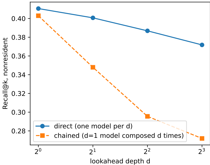
mixtral: direct vs chained lookahead
