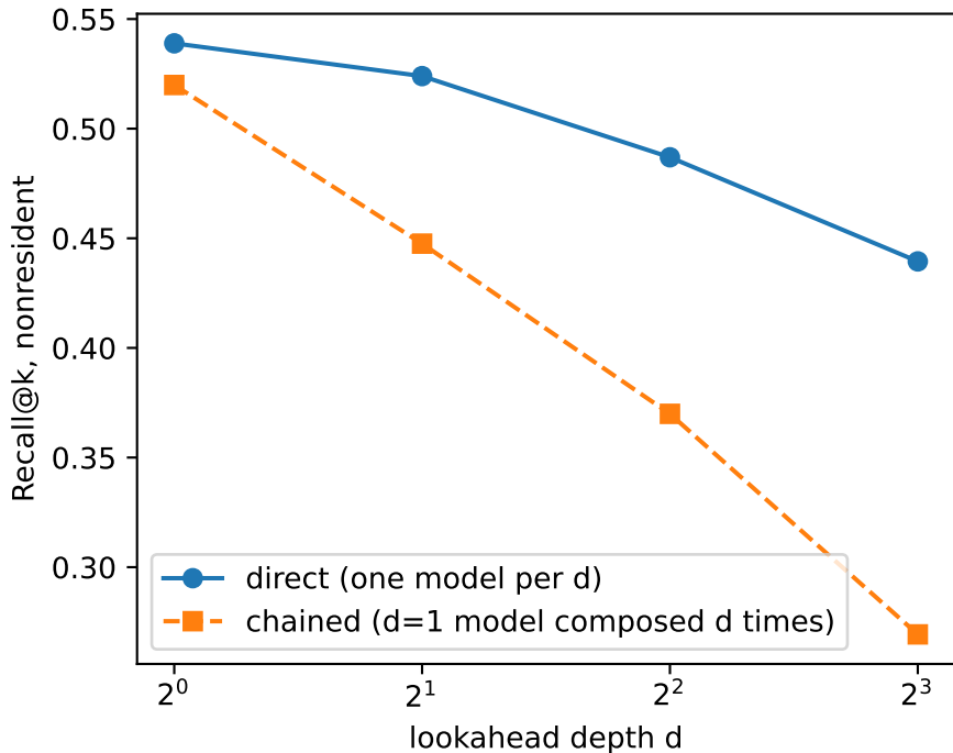
olmoe: direct vs chained lookahead
