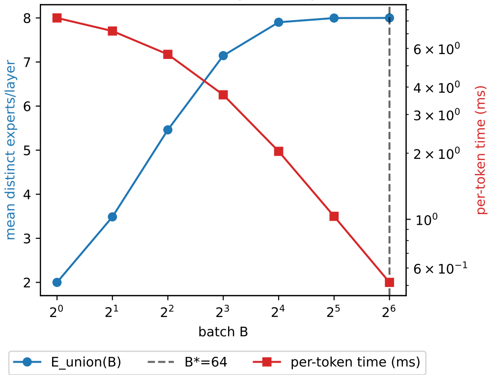
mixtral: batching sweet spot
