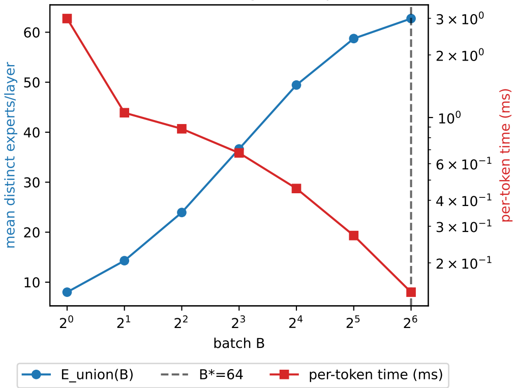
olmoe: batching sweet spot
