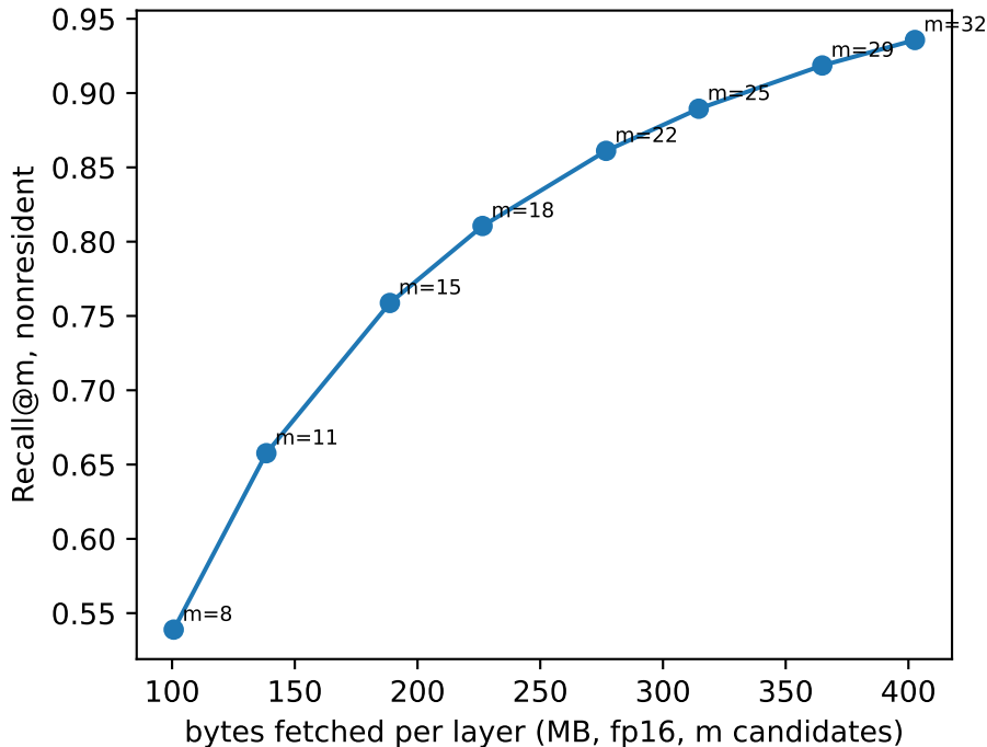
olmoe: recall vs bandwidth cost
