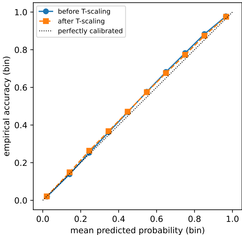
olmoe: reliability diagram
