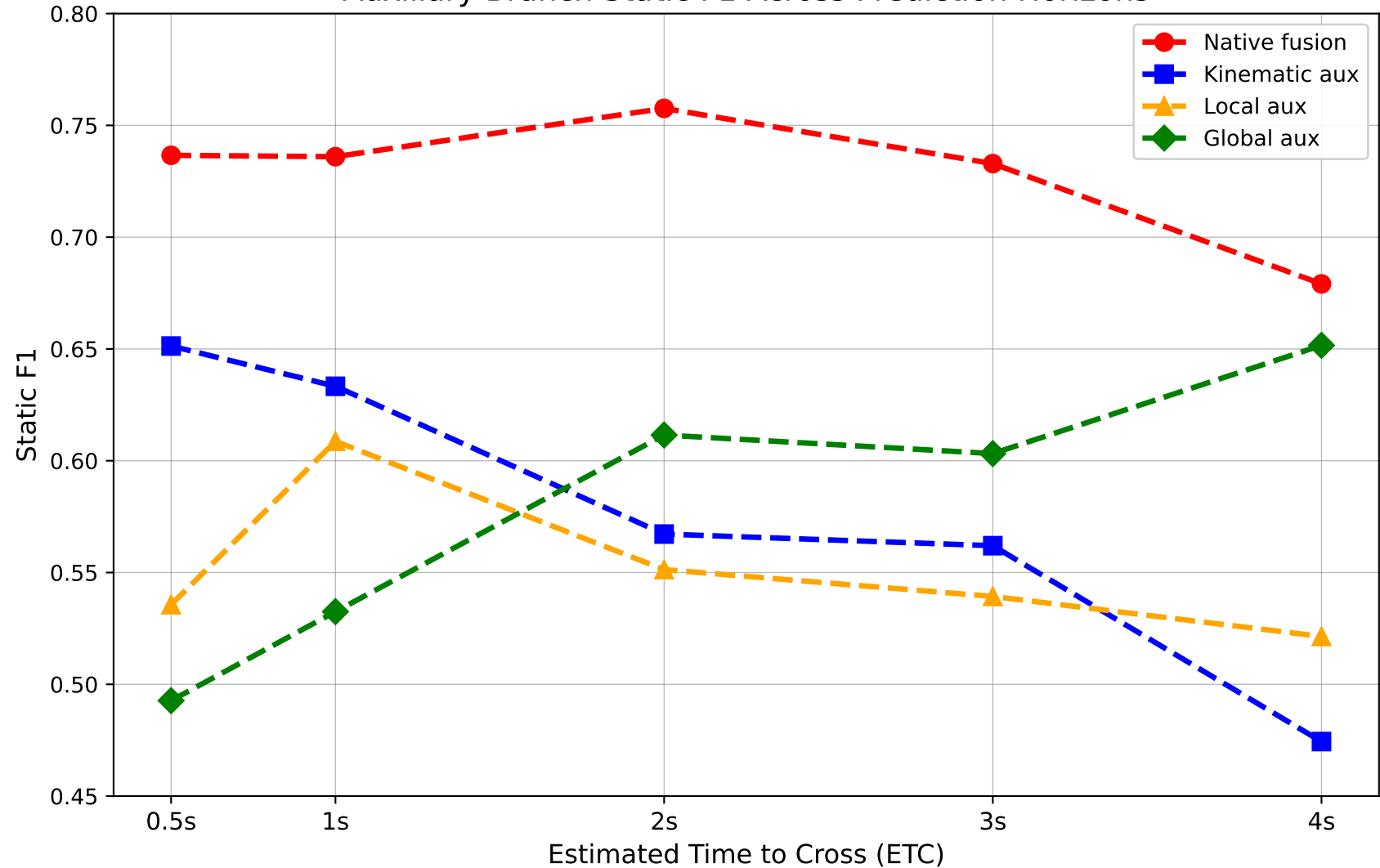
Auxiliary Branch Static F1 Across Prediction Horizons
