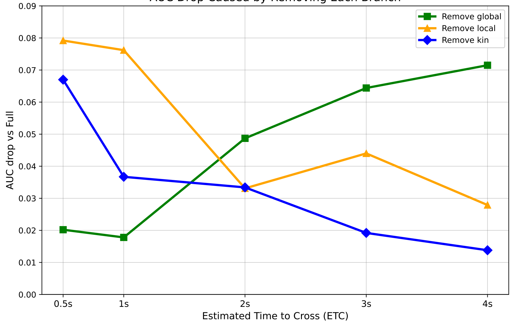
AUC Drop Caused by Removing Each Branch
