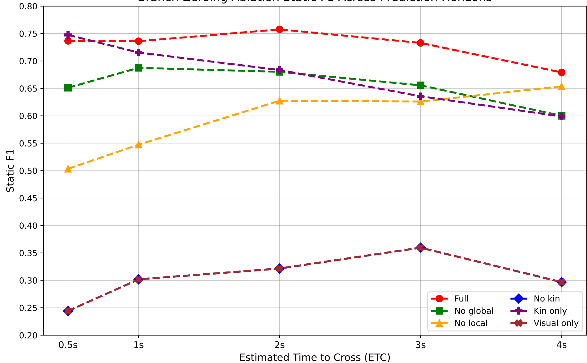
Branch-Zeroing Ablation Static F1 Across Prediction Horizons
