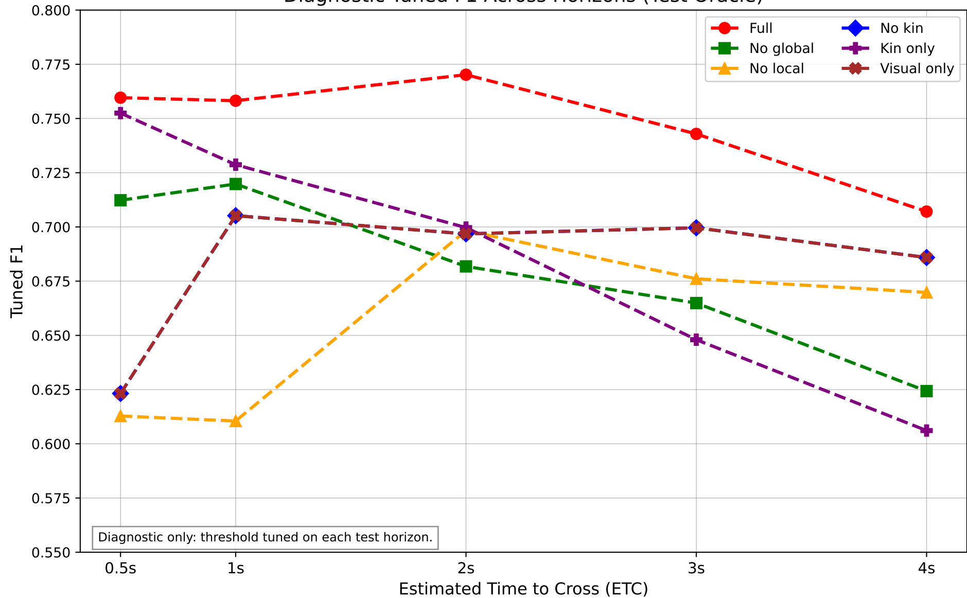
Diagnostic Tuned F1 Across Horizons (Test Oracle)
