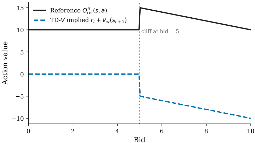
TD-V critic diagnostic near collapse (epoch 224, seed 456)
