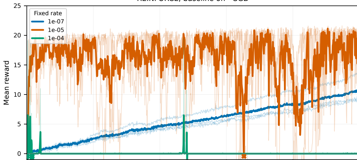
REINFORCE, baseline on - SGD
