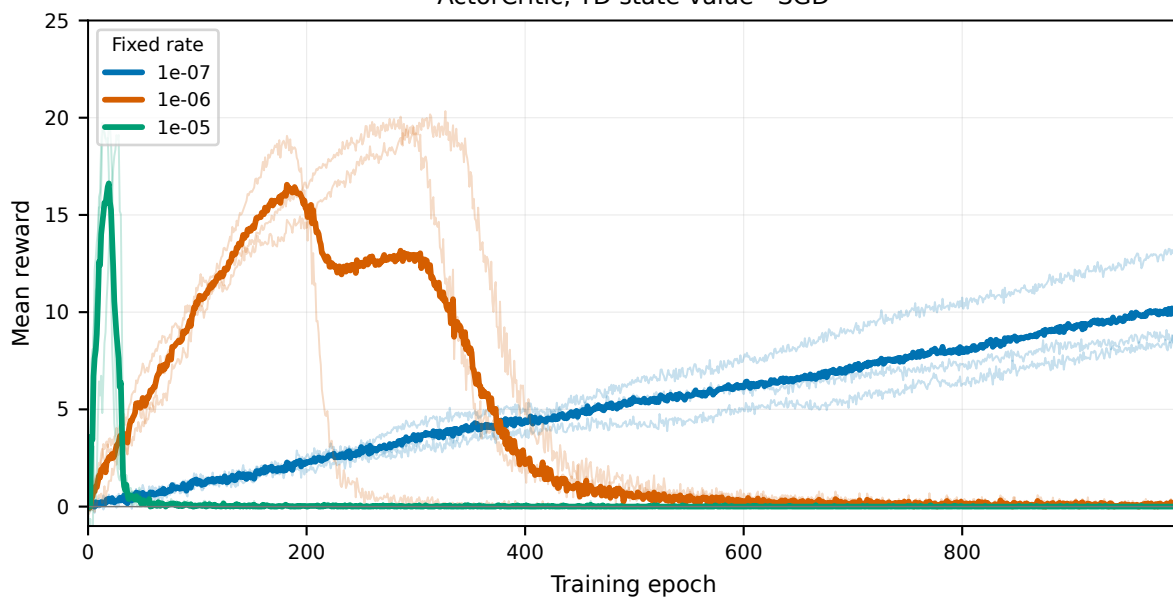
ActorCritic, TD state-value - SGD
