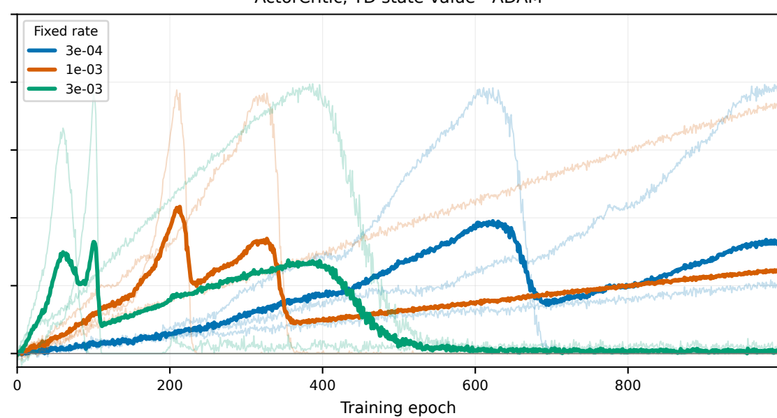
ActorCritic, TD state-value - ADAM
