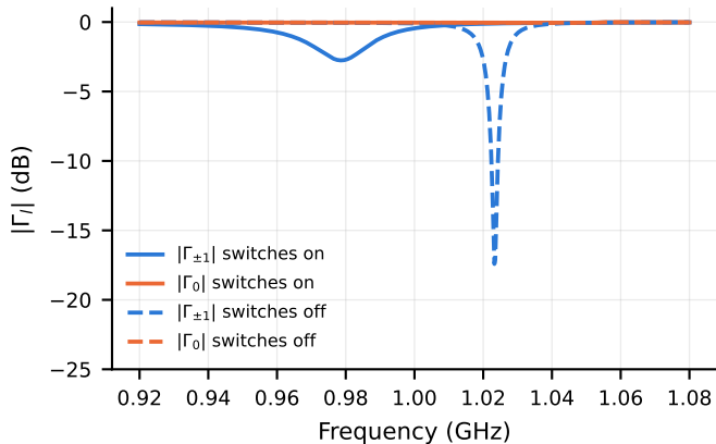
(a) Eigenmode reflection magnitude
