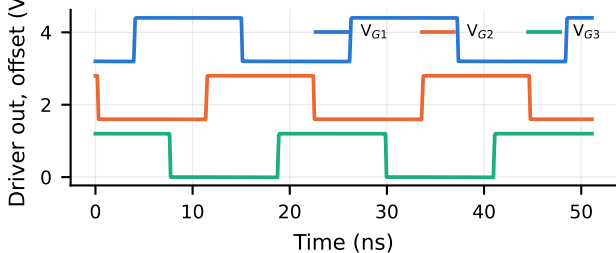
(c) Driver outputs at the switch gates
