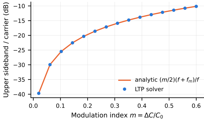
(a) Modulated-capacitor sideband check
