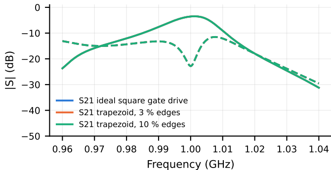
(a) Switching-edge sensitivity (solid S21, dashed S12)
