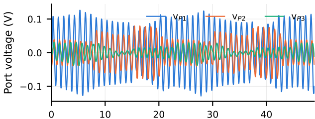
(c) Zoom: port 2 carries the signal, port 3 is isolated
