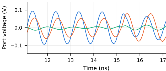
(c) Zoom: port 2 carries the signal, port 3 is isolated
