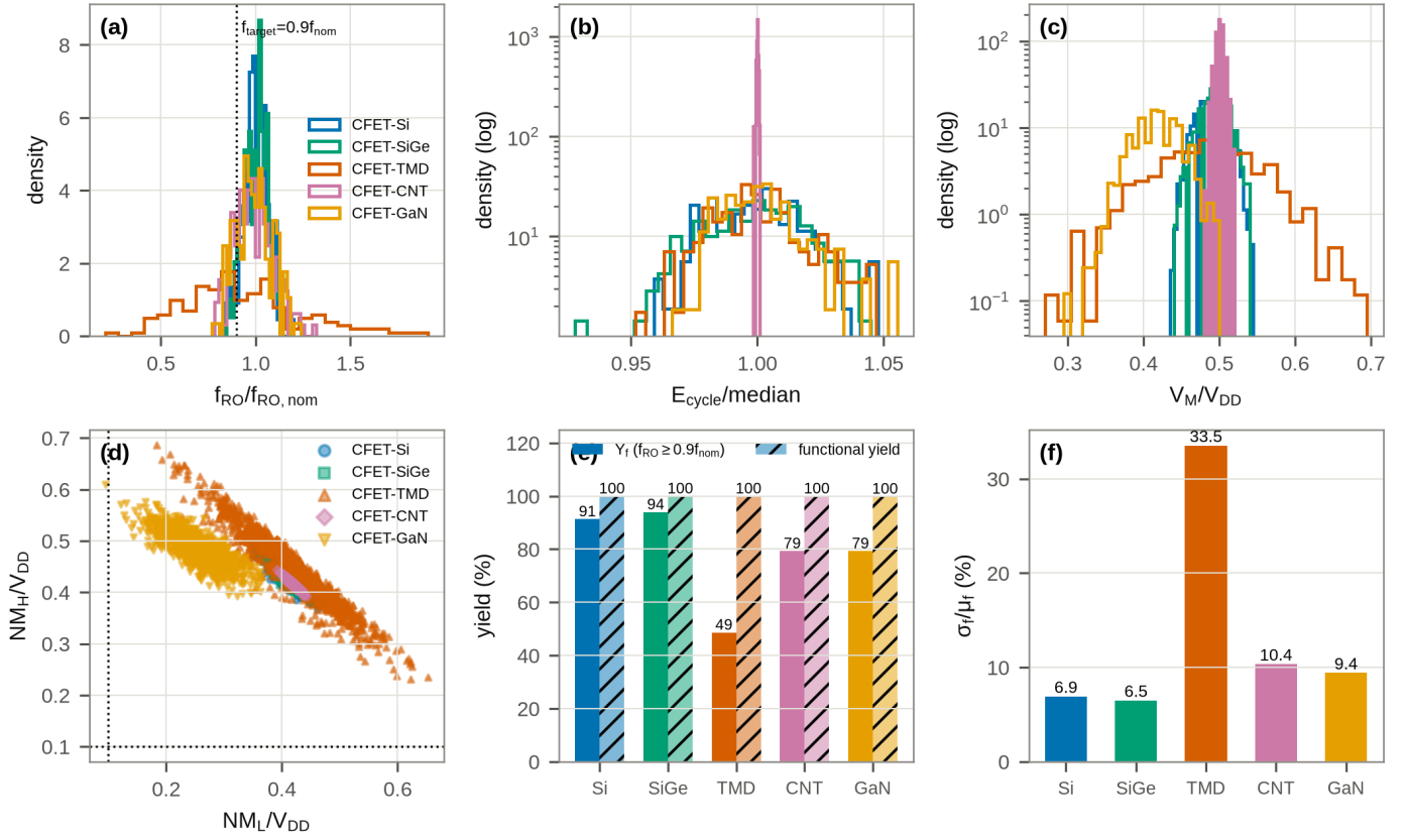
Fig. 15. Monte Carlo (200 RO samples and 1000 inverter samples per platform): (a) f_{RO} normalised to nominal, (b) energy per cycle normalised to its median, (c) V_M/V_{DD} , (d) noise-margin scatter with the 0.1V_{DD} functional limits, (e) frequency yield Y_f and functional yield, (f) relative frequency spread.
