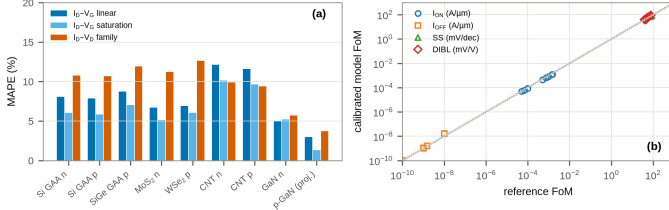
Fig. 4. (a) MAPE per device and data set; (b) parity of model vs. reference figures of merit.
