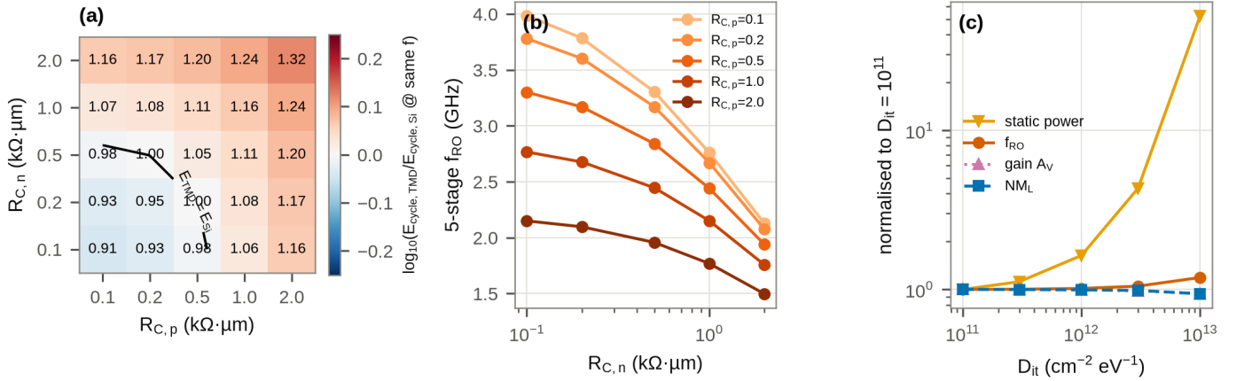
Fig. 12. TMD study: (a) iso-frequency energy-per-cycle ratio E_{TMD}/E_{Si} vs. the n- and p-contact resistance (the Si energy is interpolated at the TMD frequency from the Si V_{DD} sweep extended to 0.3 V); (b) f_{RO} vs. R_{C,n} ; (c) effect of the interface trap density.
