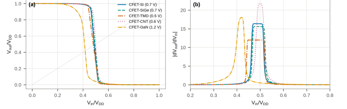
Fig. 6. (a) Normalised voltage-transfer characteristics of the five CFET inverters at their nominal V_{DD} ; (b) small-signal gain.
