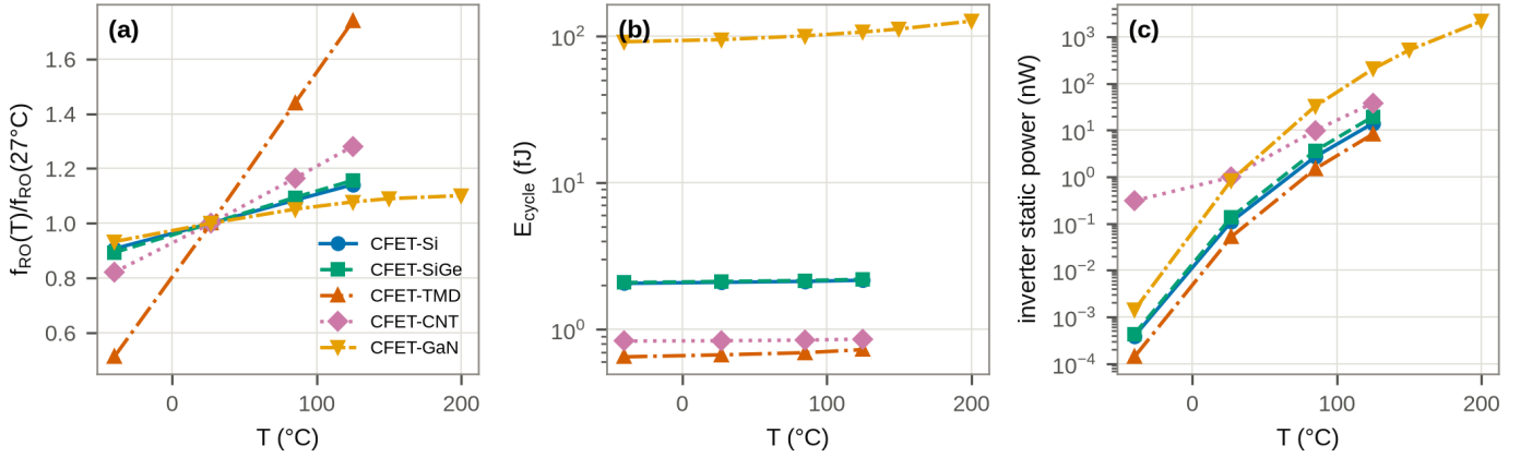
Fig. 10. Temperature sweeps at nominal V_{DD} ( -40 to 125^{\circ}\text{C} , GaN to 200^{\circ}\text{C} ): (a) normalised f_{RO} , (b) energy per cycle, (c) inverter static power.
