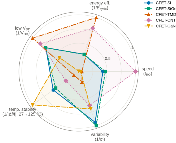
Fig. 17. Material-selection chart: speed, energy efficiency, low- V_{DD} capability, temperature stability ( 1/|\Delta f/f| between 27 and 125°C) and variability ( 1/\sigma_f ), each normalised to the best platform.
