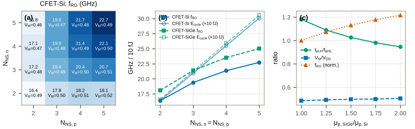
Fig. 11. Si/SiGe study: 5-stage f_{RO} and V_M/V_{DD} vs. the number of nanosheets in the n- and p-tier for (a) CFET-Si and (b) CFET-SiGe; (c) effect of the SiGe/Si hole-mobility ratio on the rise/fall delay mismatch, V_M and f_{RO} .
