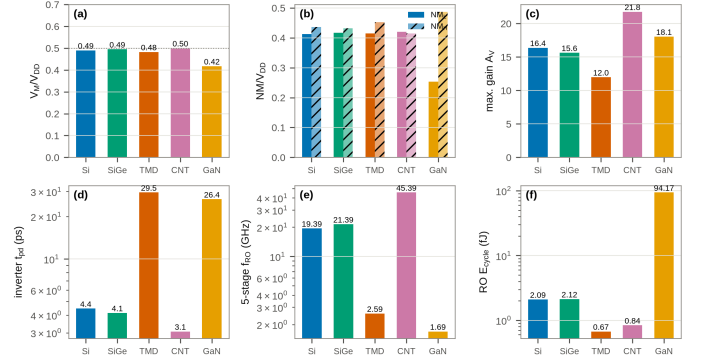
Fig. 7. Nominal figures of merit: (a) V_M/V_{DD} , (b) noise margins, (c) maximum gain, (d) inverter delay, (e) 5-stage RO frequency, (f) energy per RO cycle.
