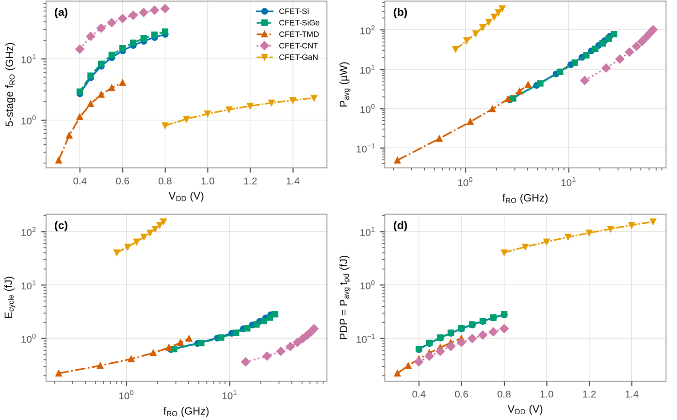
Fig. 9. Unified V_{DD} sweeps of the 5-stage ROs: (a) f_{RO} vs. V_{DD} , (b) power vs. frequency, (c) energy per cycle vs. frequency, (d) PDP vs. V_{DD} .
