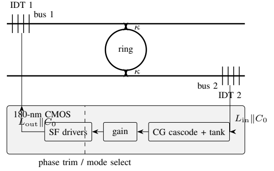
Fig. 1. Transmission-mode oscillator: the SiN–LN ring with its two IDTs closes the loop through a CMOS sustaining amplifier whose port interfaces resonate the IDT static capacitance C_0 .
