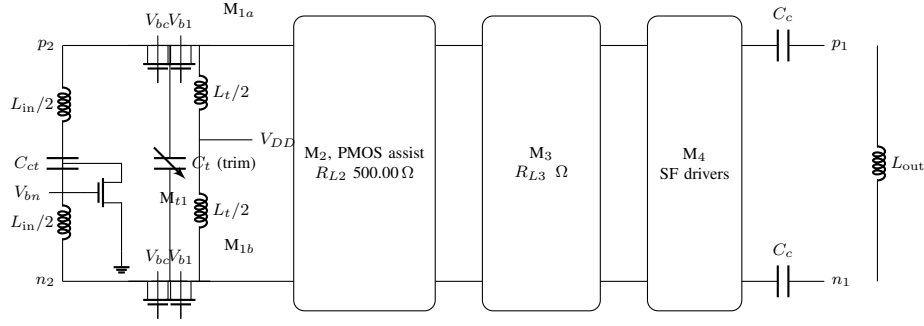
Fig. 4. Transmission-mode sustaining amplifier (one of the two symmetric halves of each stage is drawn for the CG cascode). The motional current from IDT 2 enters the common-gate pair through the centre-tapped C_0 -resonating inductor L_{in} ; the stage-1 tank with its trim varactor C_t sets the loop phase; the driver output resonates C_0 of IDT 1 with L_{out} .
