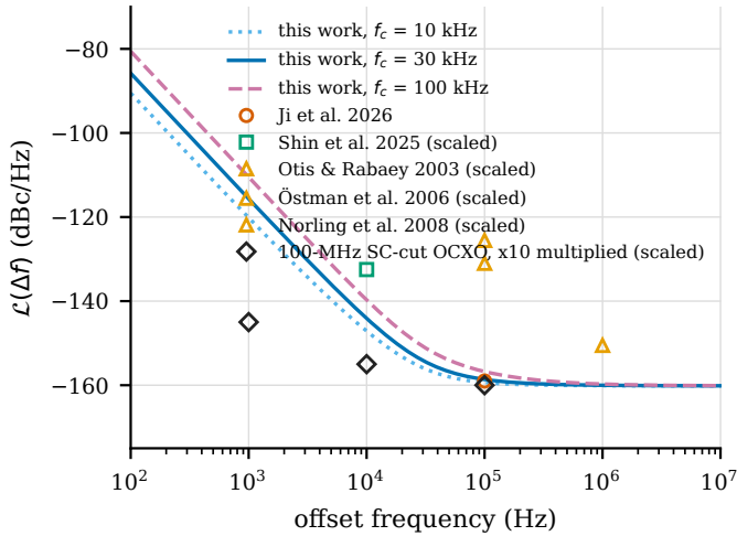
Fig. 8. Predicted phase noise (6) with circuit-derived F , Q_e and P_s for three flicker corners, compared with published SiN-LN, SAW, FBAR and quartz references (values scaled to 1 GHz by 20 \log(f_0/f_{ref}) where marked).
