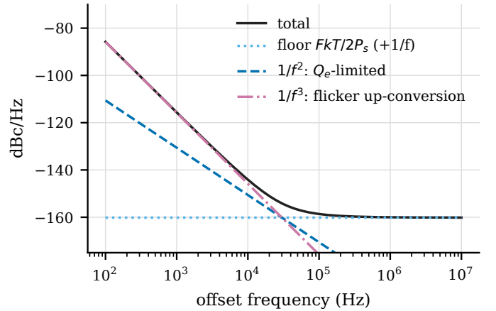
Fig. 9. Decomposition of the phase noise into the thermal floor, the Q_e -limited 1/f^2 term and the flicker 1/f^3 term ( f_c = 30 kHz).
