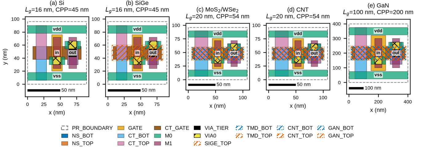
Fig. 16. Conceptual, DRC-clean GDSII layouts of the five CFET inverter cells (plan view; tiers drawn as separate layers): Si and SiGe at L_g = 16 nm, CPP = 45 nm, 90×96 nm cell; TMD and CNT projected at L_g = 20 nm, CPP = 54 nm; GaN projected at L_g = 100 nm, CPP = 200 nm.
