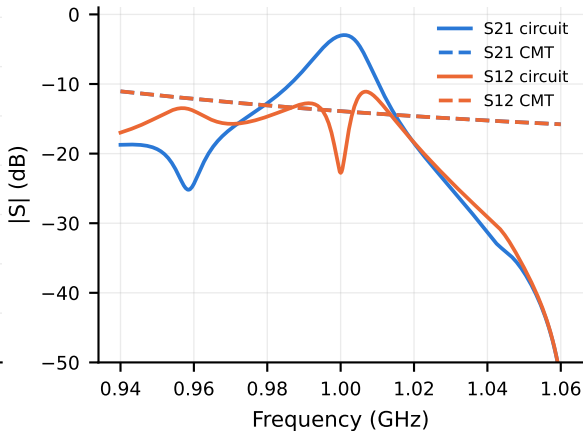
(b) Modulated: CMT vs circuit
