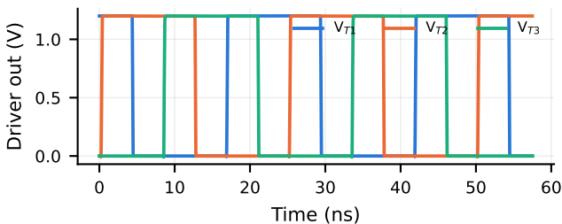
(c) Driver outputs at the switch gates
