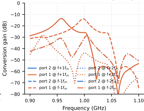
(b) Intermodulation sidebands (input at port 1)
