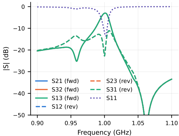
(a) Fundamental-tone S-parameters (LTP/PSP)
