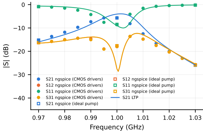
(a) Transistor-level transient vs LTP/PSP
