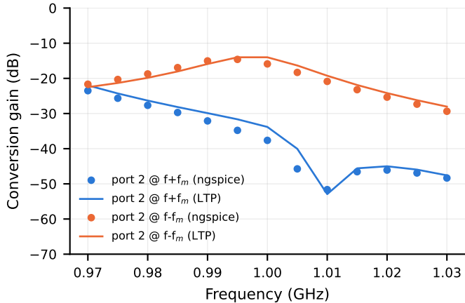
(b) Sideband conversion
