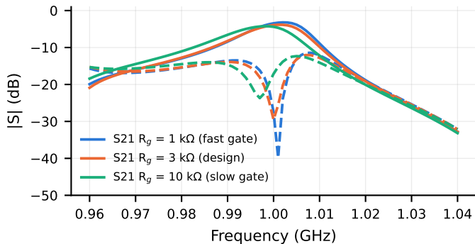
(a) Gate-edge ( R_g C_g ) sensitivity (solid S21, dashed S12)
