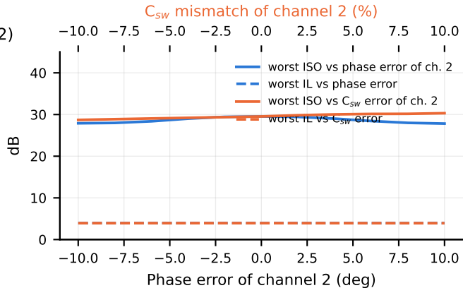
(b) Pump / element mismatch at f_0
