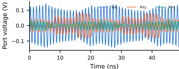
(c) Zoom: transmitted port carries the signal, isolated port does not
