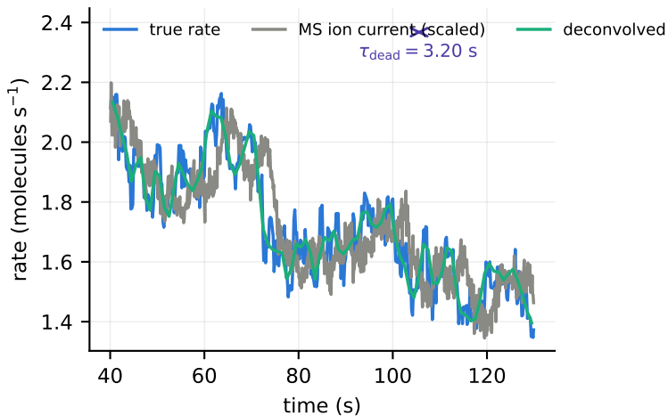
(c) transport delay and its removal
