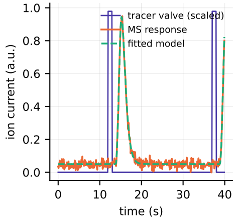
(a) tracer pulse and fit
