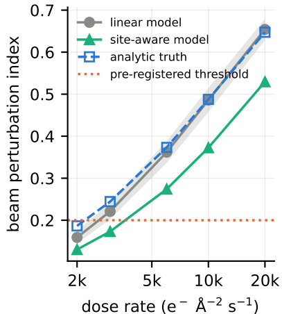
(b) BPI vs truth
