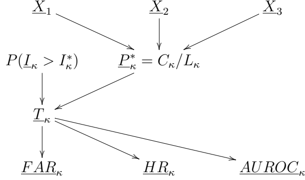
Figure 1: DAA bnet. We use one of these bnets for each \kappa value and for each grid cell of 0.25 degrees in latitude by 0.25 degrees in longitude. 1 degree in latitude or longitude is approximately 100 km.
