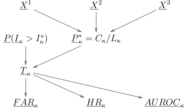
Figure 2: DAA bnet. We use one of these bnets for each \kappa value and for each grid cell of 0.25 degrees in latitude by 0.25 degrees in longitude. 1 degree in latitude or longitude is approximately 100 km.
