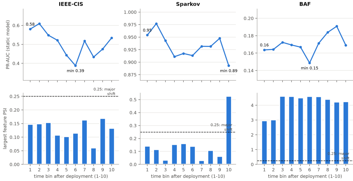
Figure 4.1: Static model after deployment, in ten consecutive time bins of the test period: PR-AUC (top) and the largest PSI among the ten most important features (bottom). Each panel has its own scale
