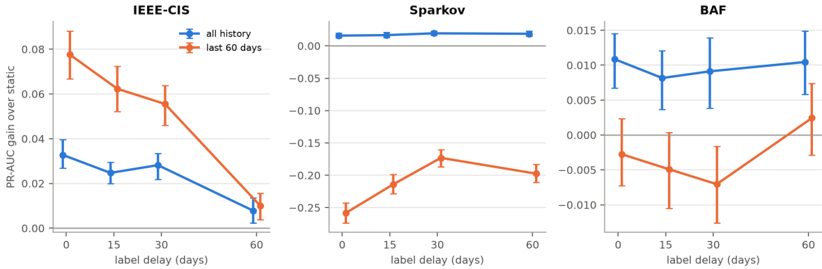
Figure 4.2: Gain in mean weekly PR-AUC over the static model for scheduled retraining every 14 days, by label delay, with 95% paired bootstrap intervals
