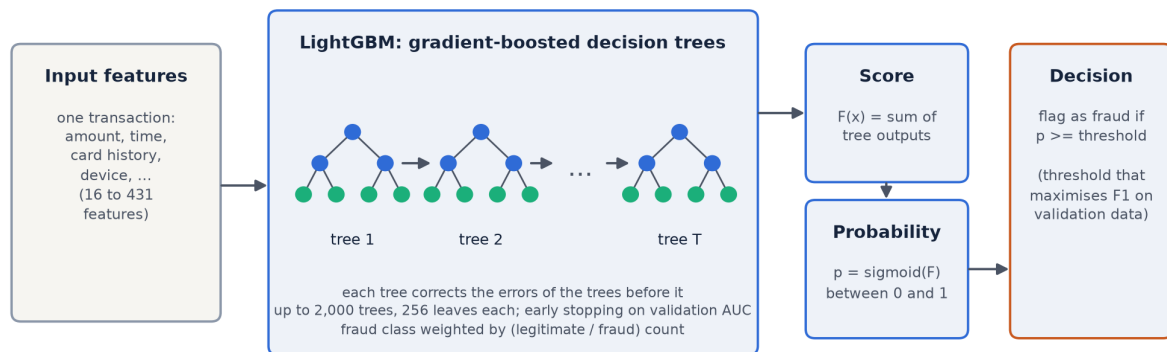
Figure 3.2: Architecture of the fraud detection model: a transaction's features pass through a sequence of boosted decision trees, whose summed output becomes a fraud probability and, with the validation threshold, a decision
