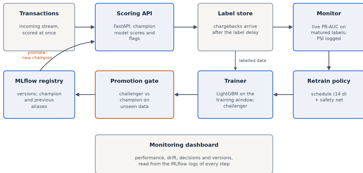
Figure 3.3: Components of the proposed framework and the flow of data between them
