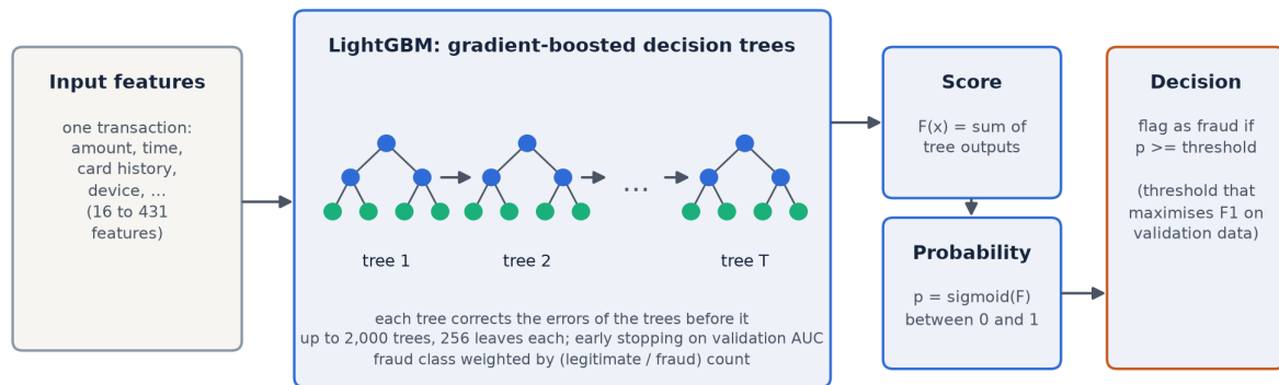
Figure 4.2: Architecture of the fraud detection model: a transaction's features pass through a sequence of boosted decision trees, whose summed output becomes a fraud probability and, with the validation threshold, a decision
