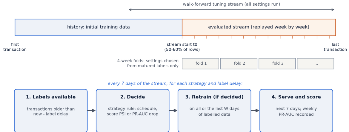
Figure 4.5: Evaluation protocol: each dataset is split in time into a history and a stream that is replayed week by week; settings are tuned walk-forward in 4-week folds
