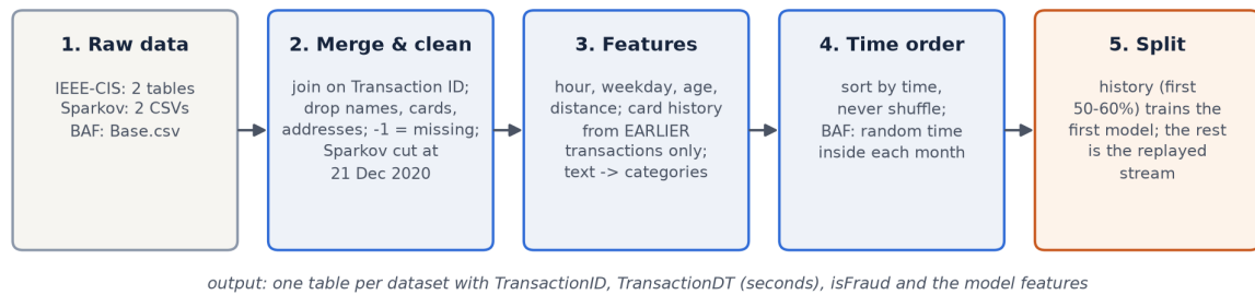
Figure 4.4: Preprocessing pipeline from the raw files of each dataset to the common time-ordered table
