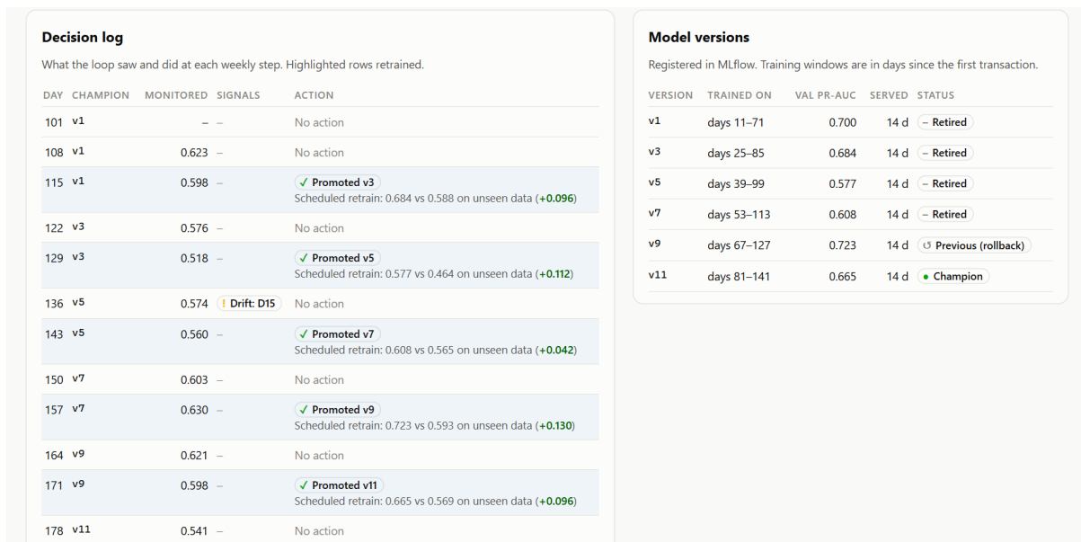
Figure 4.8: Front end: decision log and model versions on the monitoring dashboard
