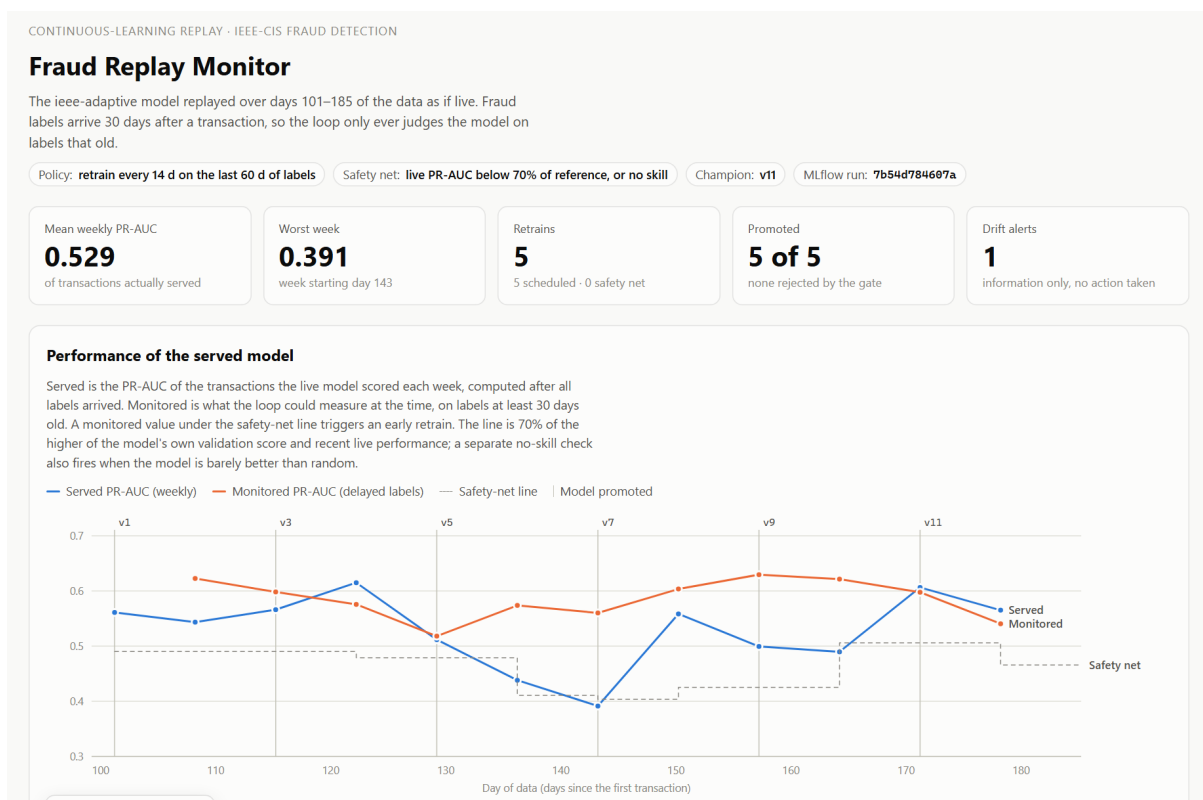
Figure 4.7: Front end: the monitoring dashboard after a replay of IEEE-CIS (summary figures and the performance of the served model)
