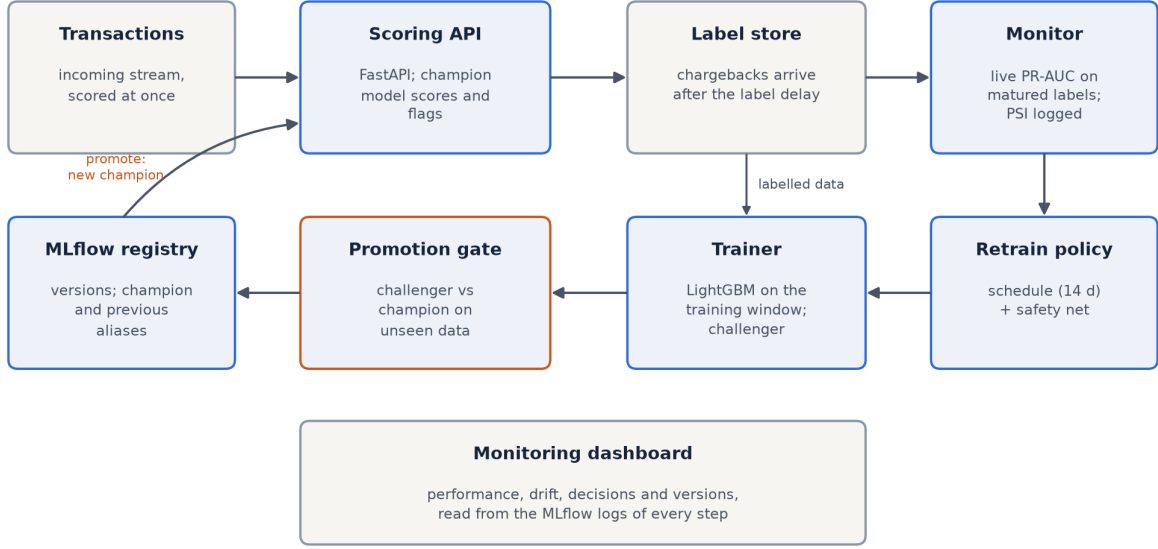
Figure 4.3: Components of the proposed framework and the flow of data between them
