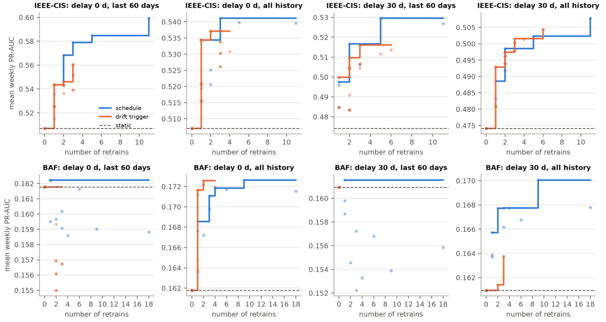
Figure 5.3: Equal-budget comparison on IEEE-CIS (top) and BAF (bottom): the best mean weekly PR-AUC each family reaches with at most a given number of retrains (dots: individual settings)
