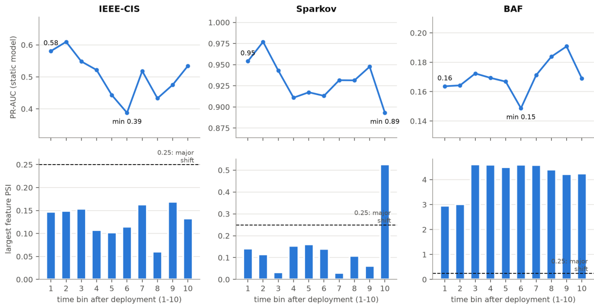
Figure 5.1: Static model after deployment, in ten consecutive time bins of the test period: PR-AUC (top) and the largest PSI among the ten most important features (bottom). Each panel has its own scale
