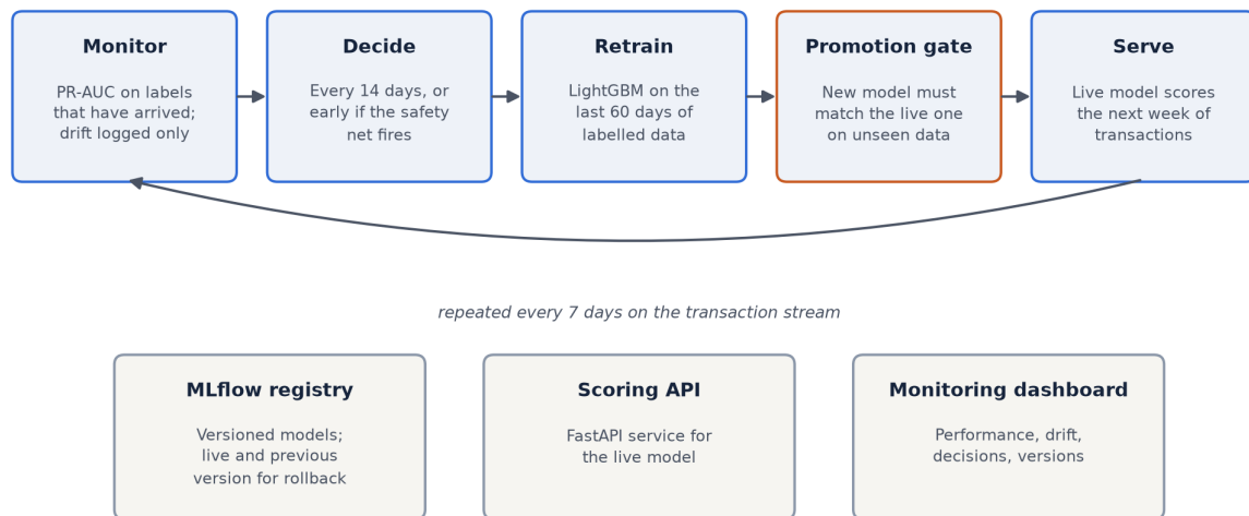
Figure 4.4: The proposed continuous-learning loop, run every week on the transaction stream
