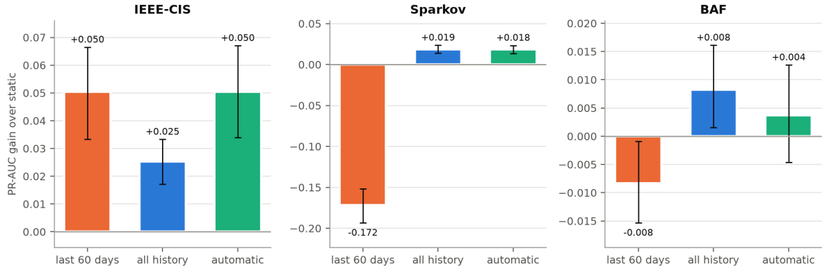
Figure 5.5: Framework replays (30-day label delay): gain in mean weekly PR-AUC over the static model for each training-window choice, with 95% bootstrap intervals over weeks
