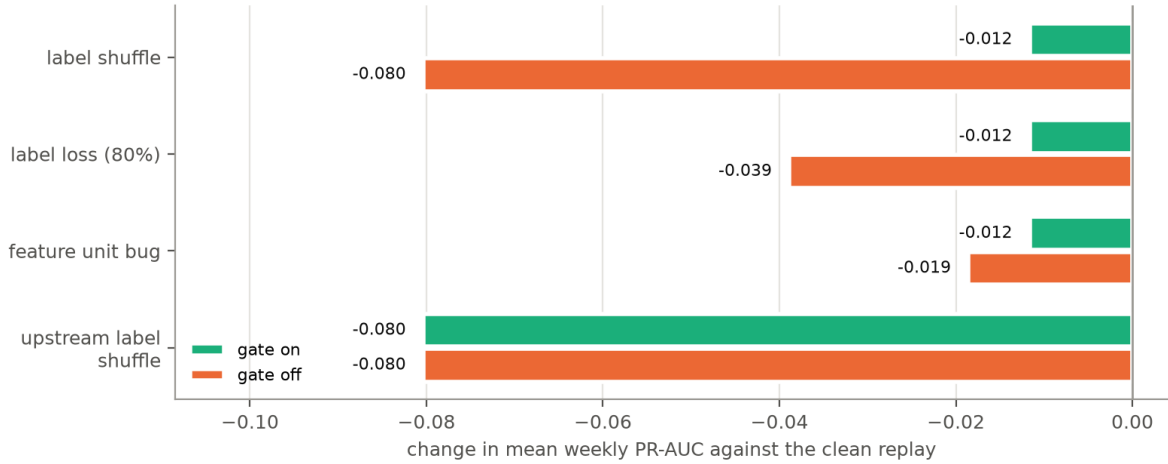
Figure 5.4: Fault injection on IEEE-CIS: change in mean weekly PR-AUC against a clean replay when two retraining jobs are faulty, with the promotion gate on and off
