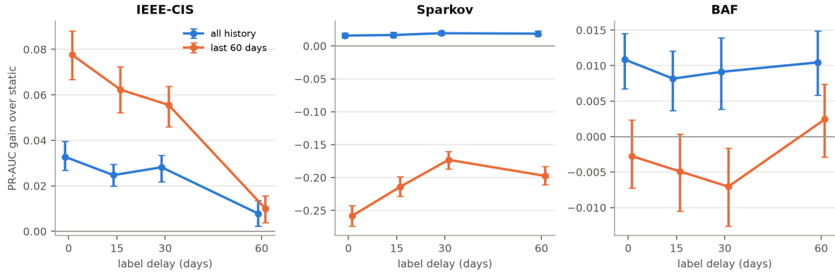
Figure 5.2: Gain in mean weekly PR-AUC over the static model for scheduled retraining every 14 days, by label delay, with 95% paired bootstrap intervals
