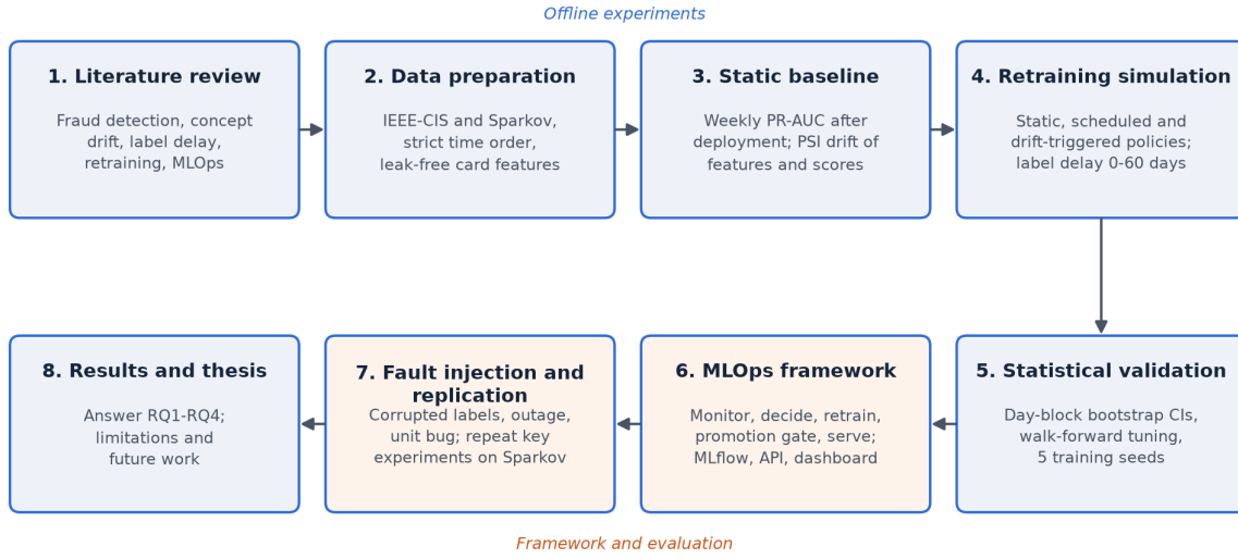
Figure 4.2: Methodology of the study: from literature review and time-ordered data preparation to the retraining experiments, the framework and its evaluation
