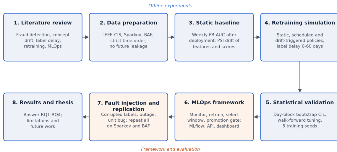
Figure 4.1: Methodology overview: the experiments on three datasets, the framework and its evaluation
