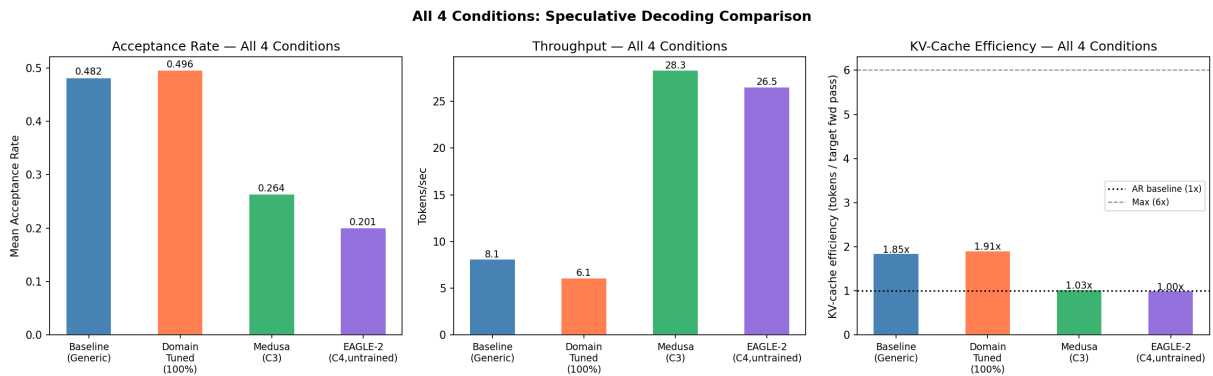
Figure 4: Side-by-side comparison of all four conditions — acceptance rate (left), throughput in tokens/sec (centre), and KV-cache efficiency/speedup (right).
