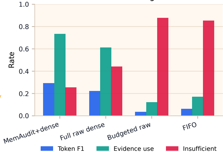
Frozen-reader diagnostic
