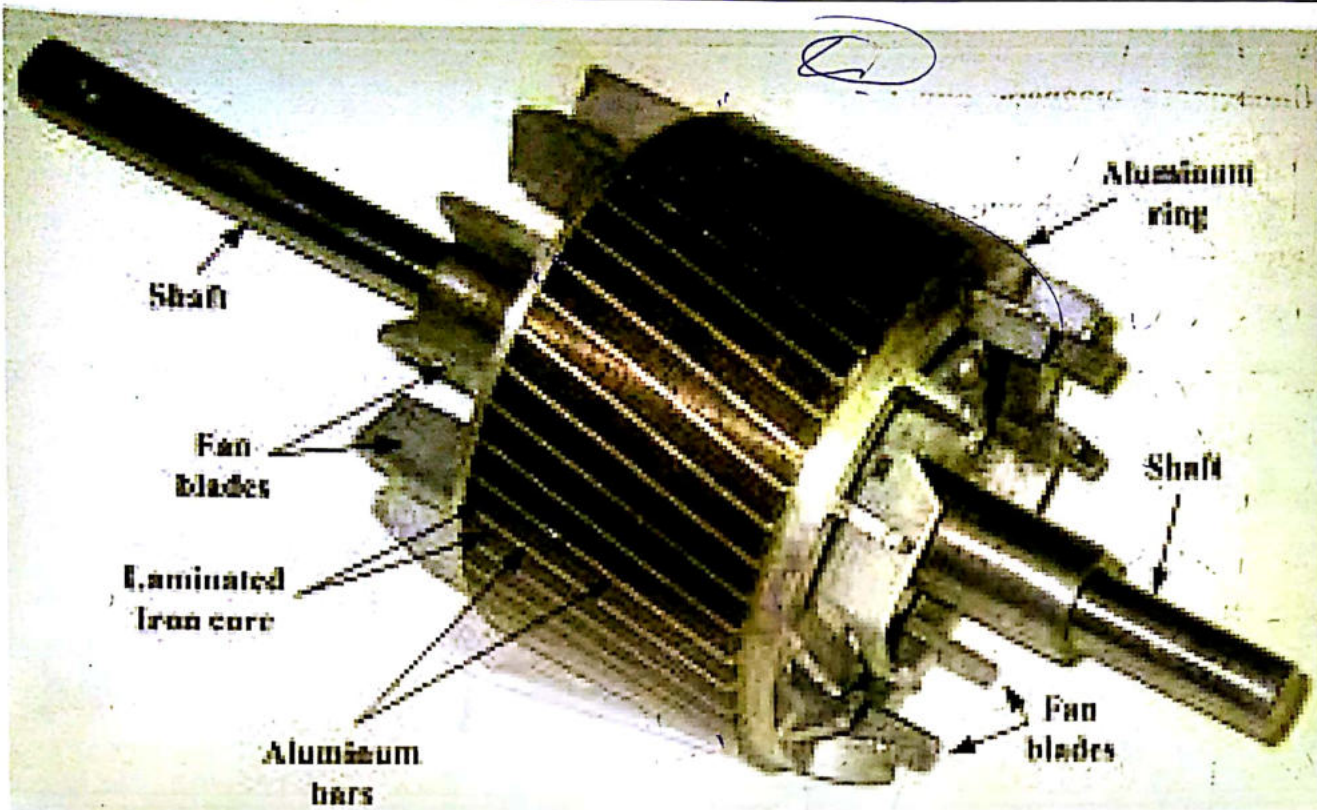
Squirrel cage Rotor
