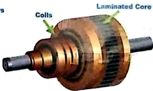
Wound Rotor
