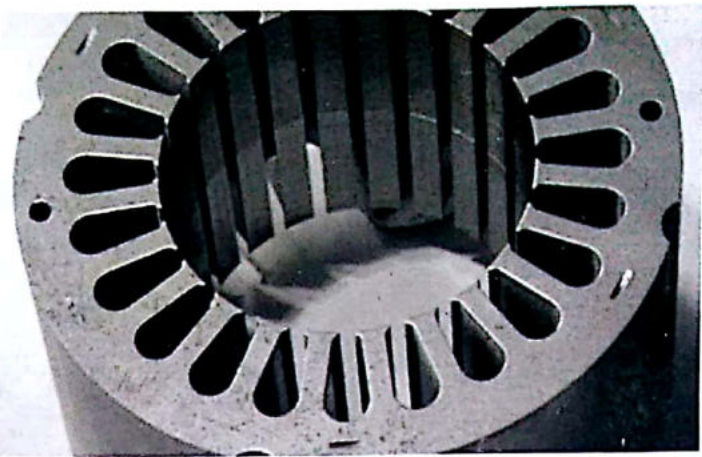
Open slots
