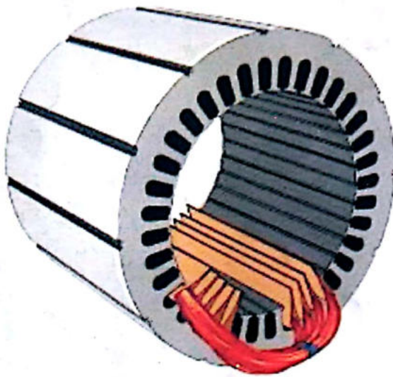
Stator Windings Partially Completed
